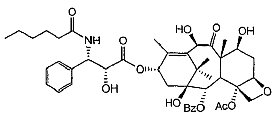
10-Deacetyltaxol C
