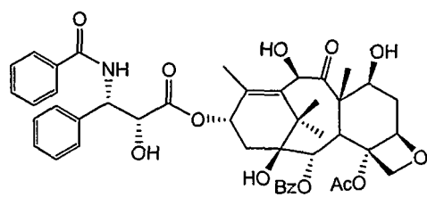
10-Deacetyltaxol A
