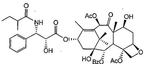
Taxol E
