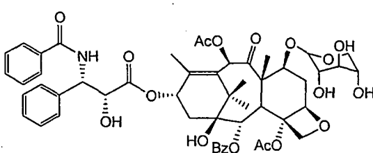
7-Xylosyltaxol A
