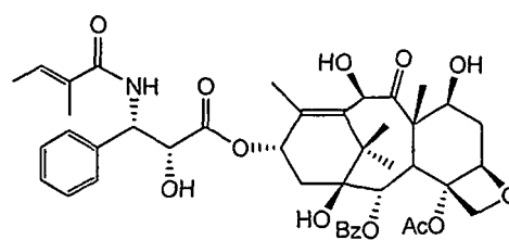
10-Deacetyltaxol B
