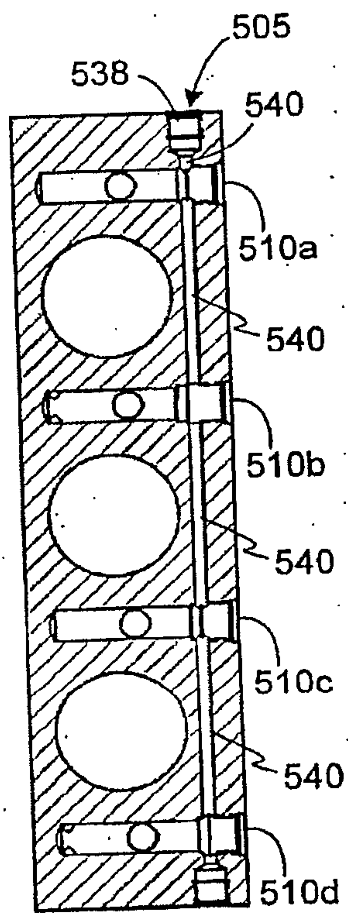
SECTION C-C FIG. 10C
