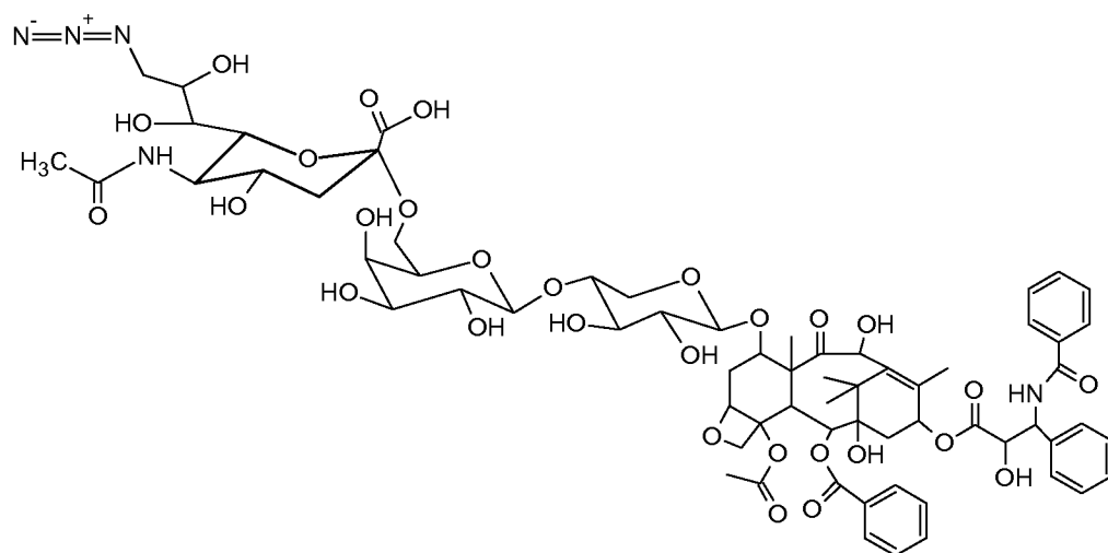
Scheme 11. Structure of 9-N 3 -NeuAcα2,6Galβ1,4Xyl-taxol
