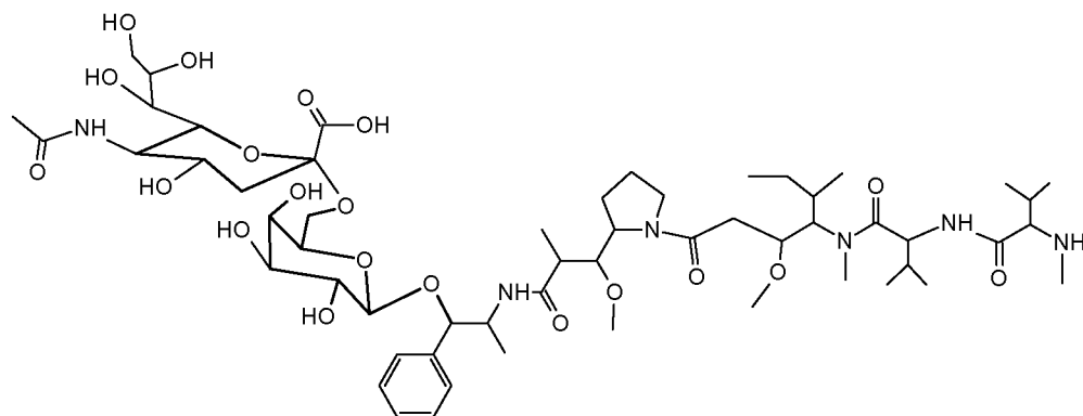
Scheme 22. Structure of Neu5Ac \alpha 2,6MMAG
