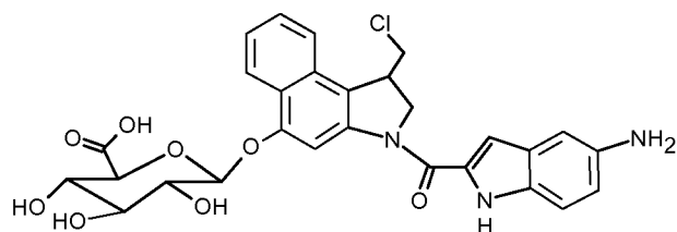
Scheme 33. Structure of glucuronyl duocarmycin.
