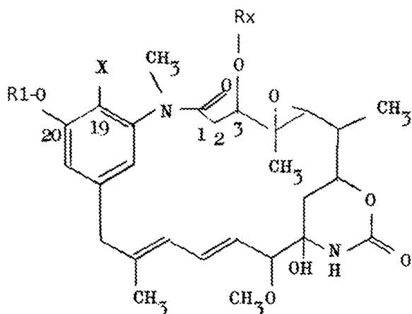
Scheme 38. X is Cl or H; R1 is H or saccharide; Rx is H or acyl group.
