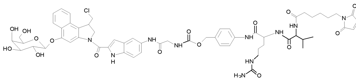
Scheme 31. Structure of Gal-Duocarmycin-PAB-CV-maleimide.
