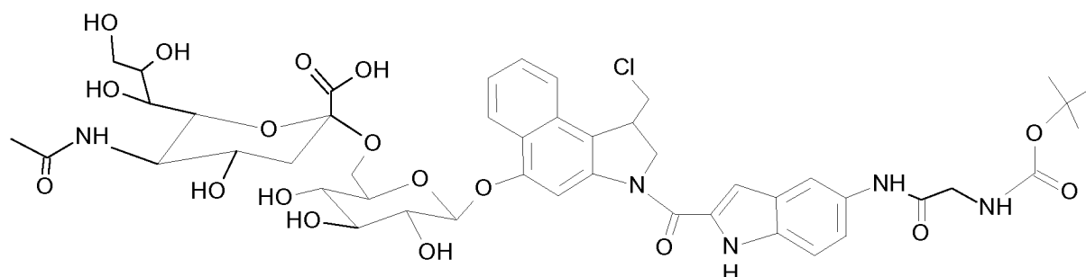
Scheme 19. Structure of Neu5Ac \alpha 2,6Gal-Duocarmycin
