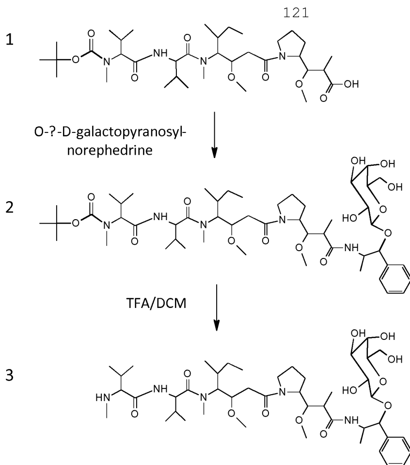
Scheme 2. Synthesis of O-β-D-galactopyranosylmonomethylauristatin E (MMAG)
