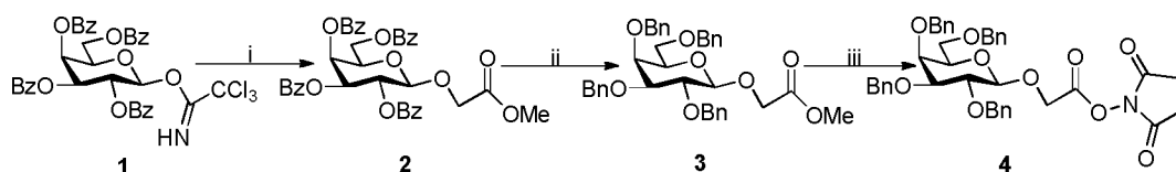
Scheme 28. i) Methyl glycolate, TMSOTf, DCM; ii) 1) NaOMe, MeOH; 2) NaH, BnBr, DMF; iii) 1) NaOMe, MeOH:H 2 O; 2) NHS, EDC, DMF.
