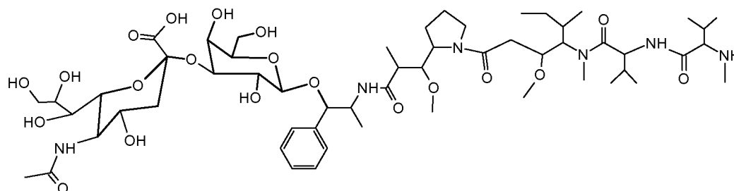
Scheme 23. Structure of Neu5Acα2,3MMAG
