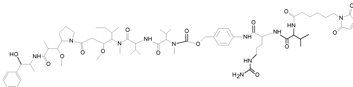
Scheme 25. Structure of maleimidocaproyl-VC-PAB-MMAE.
