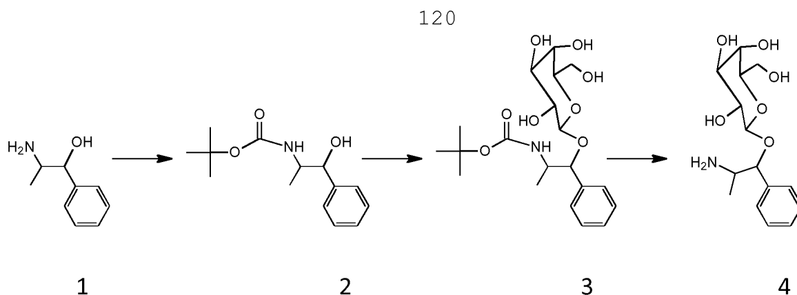
Scheme 1. Synthesis of O-β-D-galactopyranosyl-norephedrine
