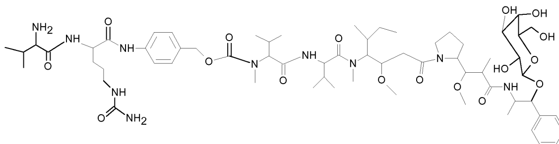
Scheme 5. Structure of Val-Cit-PAB-(O-β-D-galactopyranosyl)monomethylauristatin E
