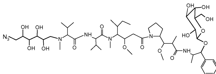
Scheme 4. Structure of N-(6-azido-6-deoxy-D-galactos-yl)-O-β-D-galactopyranosylmonomethylauristatin E
