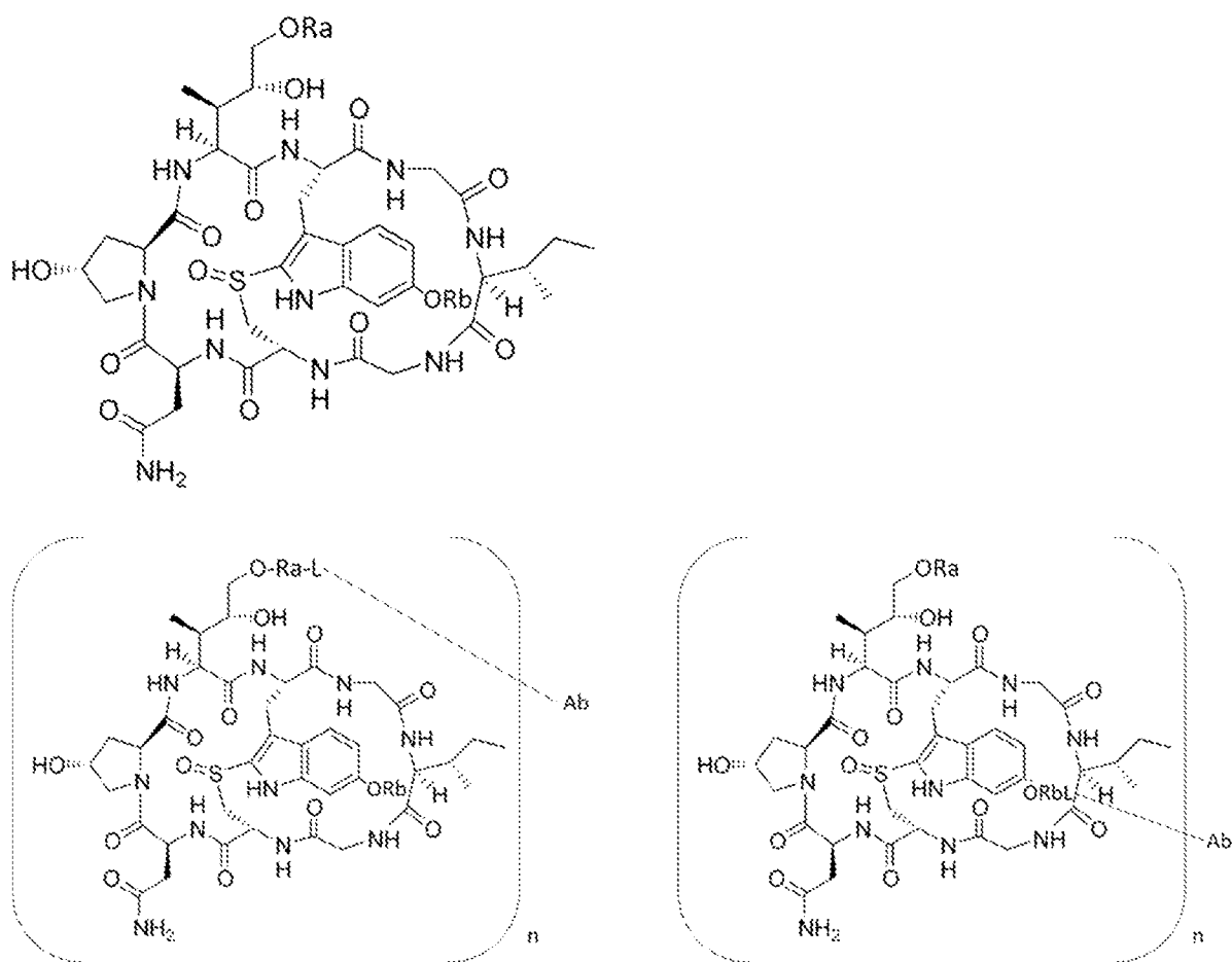
Scheme 43. Ra is H, saccharide, or L-Ab; Rb is H, saccharide, or L-Ab; and Ra \neq Rb. L may be absent or any linker group described
