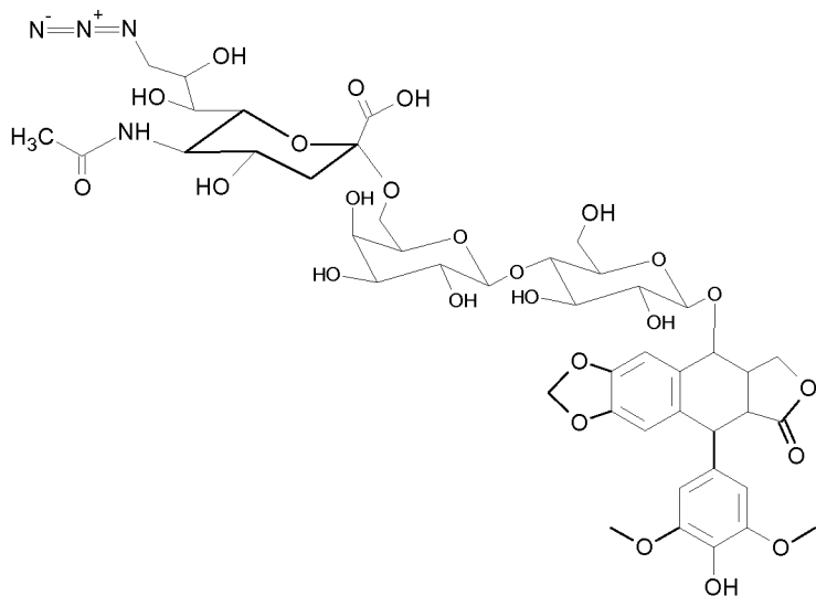
Scheme 7. 9-azido-sialyl derivative of beta-D-4'-demethylepipodophyllotoxin glucopyranoside
