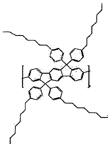
Polyidenofluorene, aryl-octyl side chains
