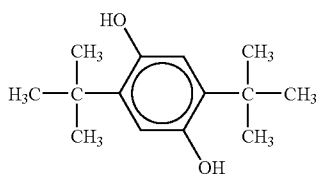
2,6-Di-tert-butyl-p-cresol: a compound represented by the formula below
