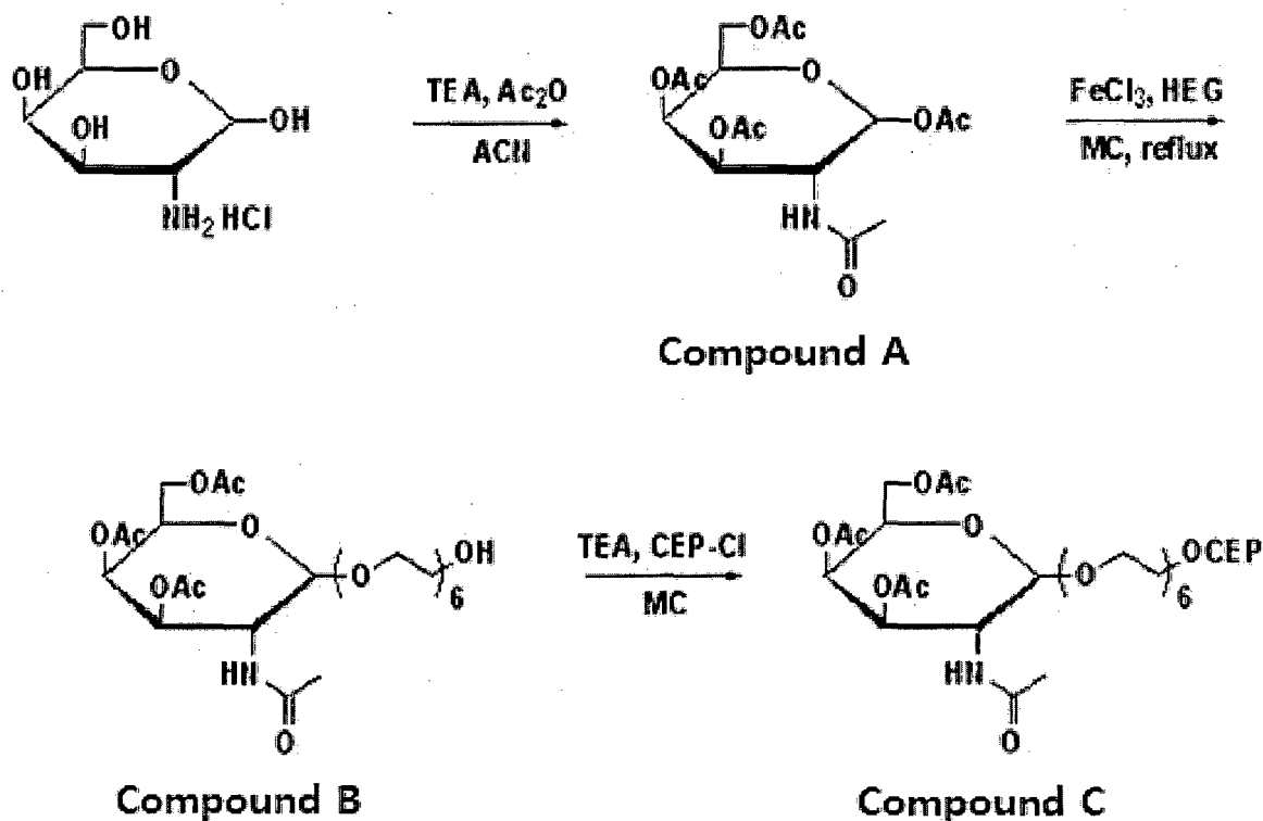
Reaction scheme 1
