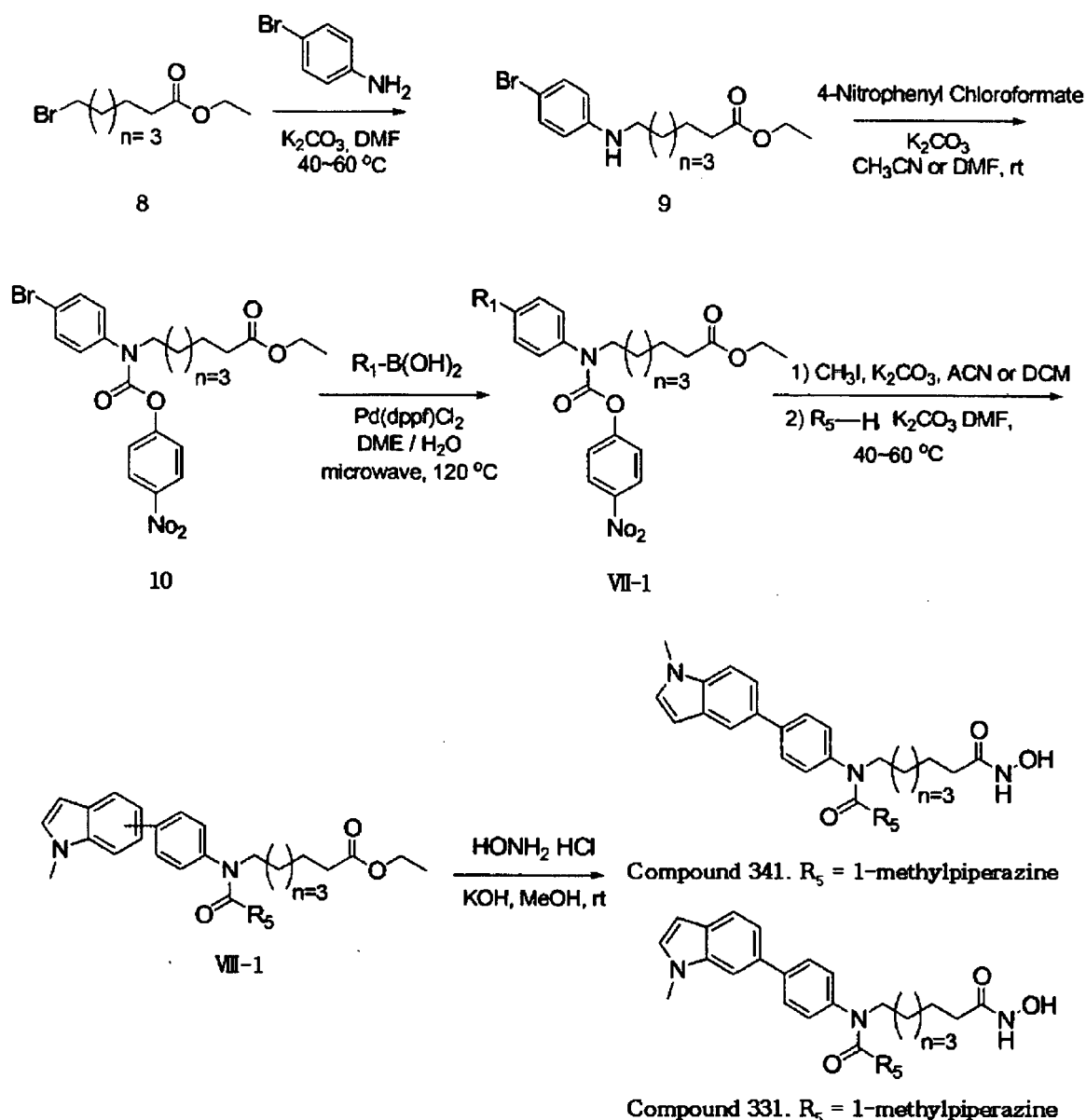
[Reaction Scheme 6]
