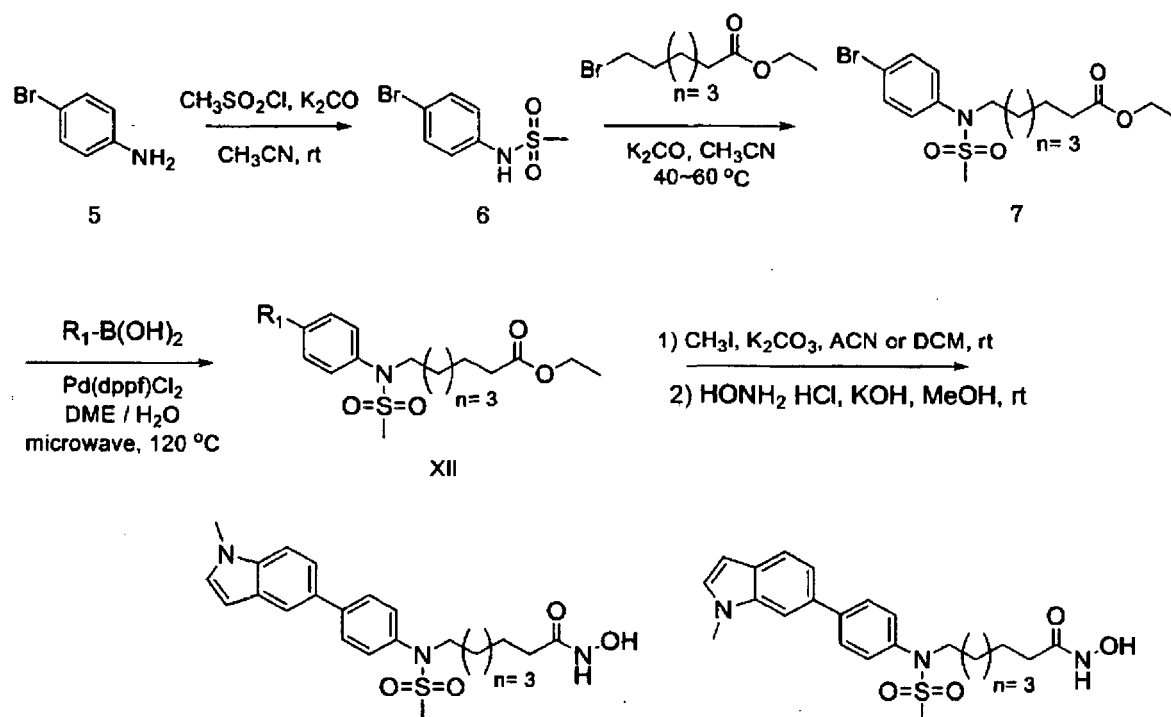
Compound 320. \text{R}_1 = 1\text{H-indol-5-yl}
