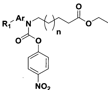
[Formel VIII]
