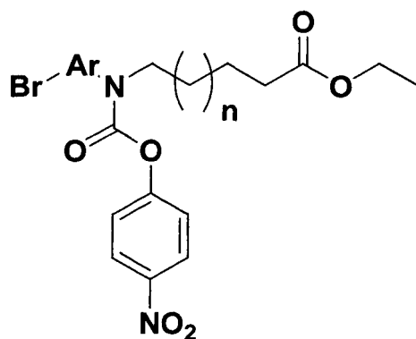
[Formel VI]
