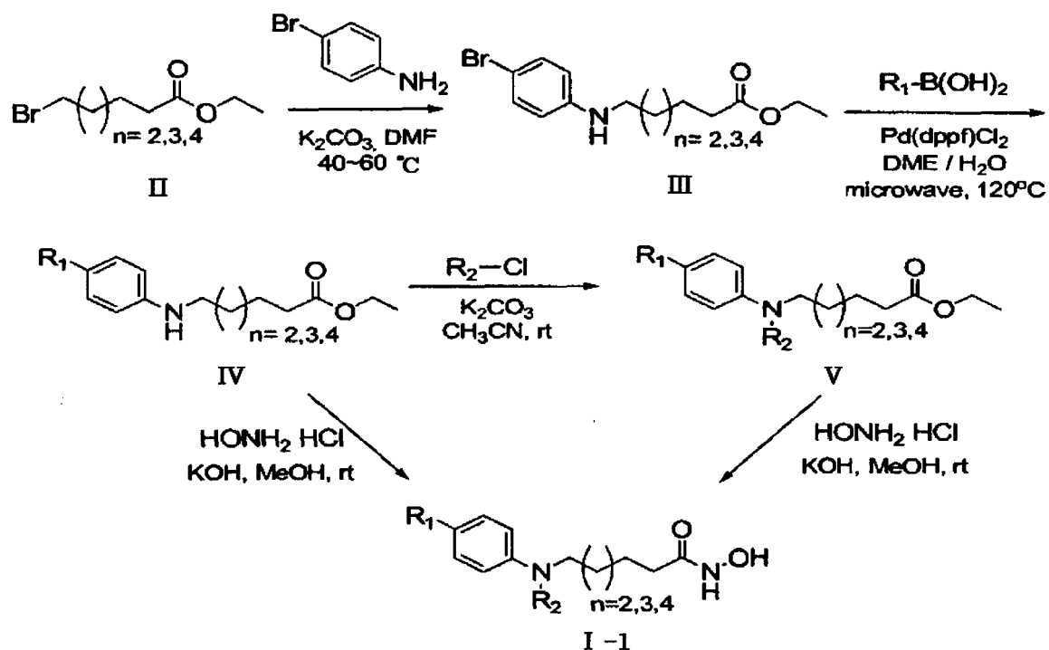
[Reaction Scheme 1]
