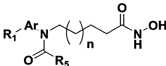
[Formula I-2]
