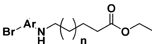
[Formula III]
