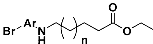
[Formula III]
