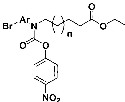
[Formula VI]
