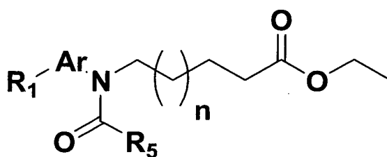
[Formel VIII]
