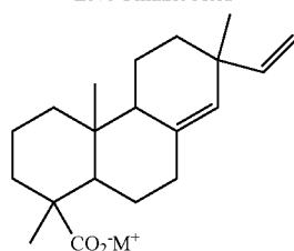
Sandaracopimaric Acid
