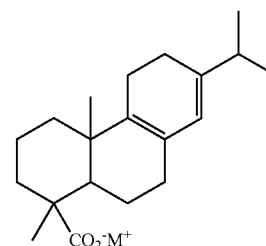
Palustric Acid
