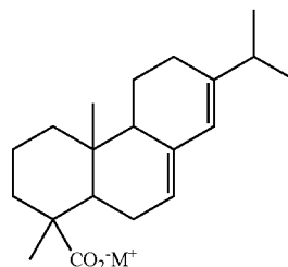
Abietic Acid
