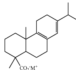
Palustric Acid
