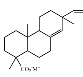
Pimaric Acid
