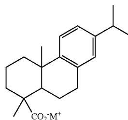
Dehydroabietic Acid
