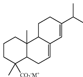
Abietic Acid
