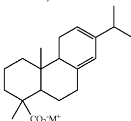
Levo-Pimaric Acid
