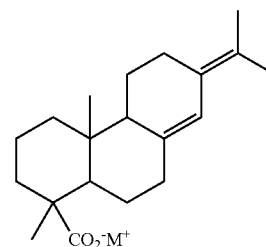
Neo-Abietic Acid
