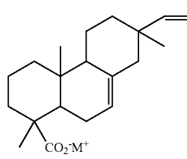
Iso-Pimaric Acid
