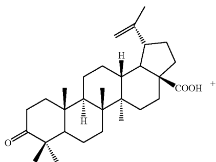
betulonic acid 1 \text{C}_{30}\text{H}_{46}\text{O}_3
