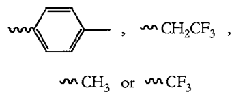
PAG sulfonates, wherein R =
