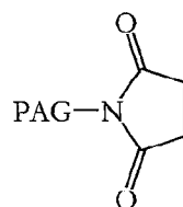
PAG maleimide derivative
