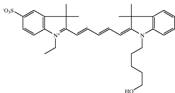
1-Ethyl-2-{5-[1-(5-hydroxypentyl)-3,3-dimethyl-2,3-dihydro-1H-benzo[b]azol-2-yliden]-1,3-pentadienyl}-3,3-dimethyl-3H-benzo[b]azolium-5-sulfonate
