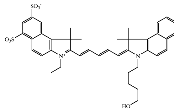
Potassium 3-ethyl-2-{5-[3-(5-hydroxypentyl)-1,1-dimethyl-2,3-dihydro-1H-naphtho[2,1-b]azol-2-yliden]-1,3-pentadienyl}-1,1-dimethyl-1H-naphtho[2,1-b]azolium-6,8-disulfonate
