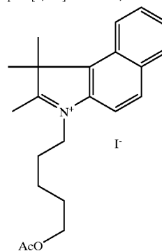
1,1,2-Trimethyl-3-(5-methylcarbonyloxypentyl)-1H-naphtho[2,1-b]azolium iodide
