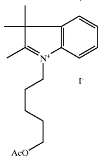
2,3,3-Trimethyl-1-(5-methylcarbonyloxypentyl)-3H-benzo[b]azolium iodide
