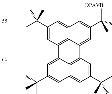
TBPc
