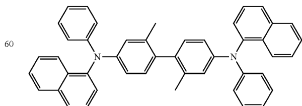
methylated NPB
