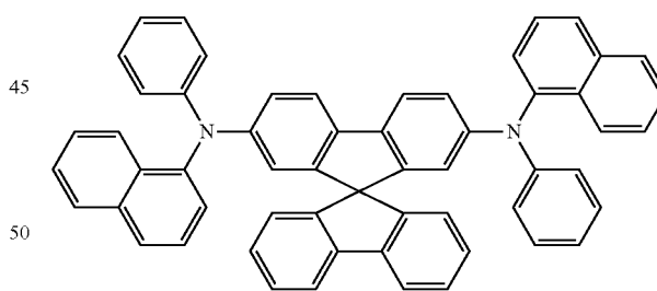
Spiro-NPB
