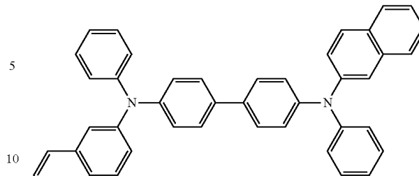
\beta -NPB
