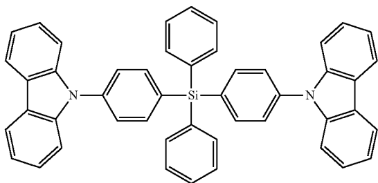
BCPDS
