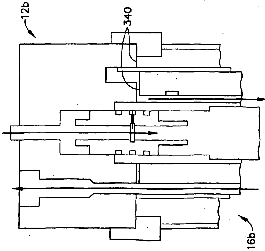
FIG. 32a (COOLING FLUID PASSAGEWAYS)
