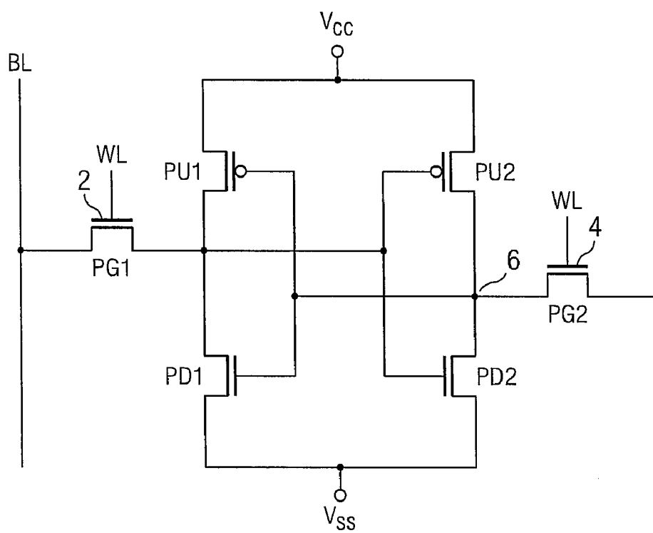
FIG. 1 (PRIOR ART)
