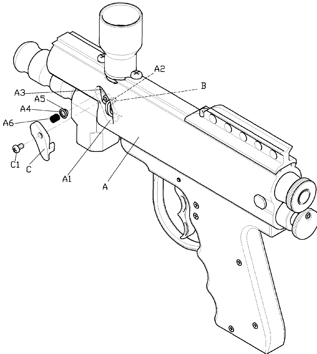
FIG. 6 (PRIOR ART)
