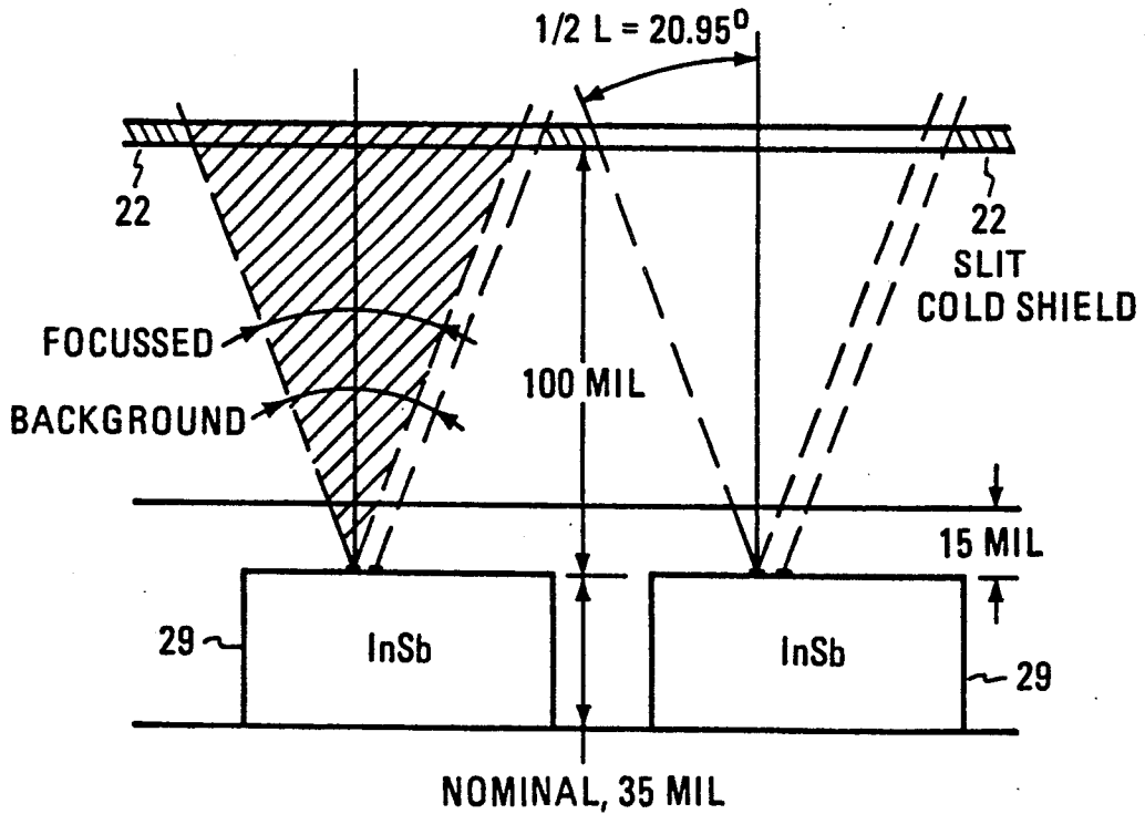
FIG. 3C PIXEL ANGULAR FIELD IN OPTICAL SCAN DIRECTION
