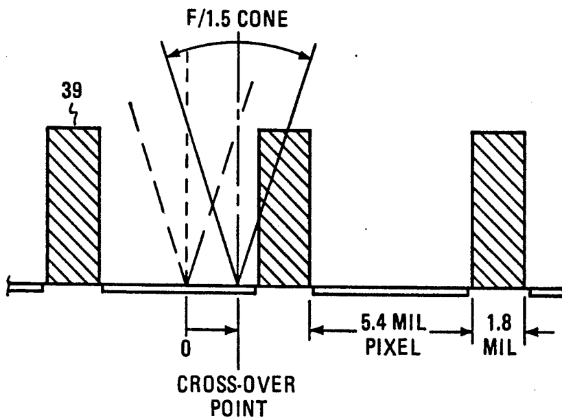
FIG. 5B PIXEL ANGULAR FIELD IN RESOLUTION DIRECTION
