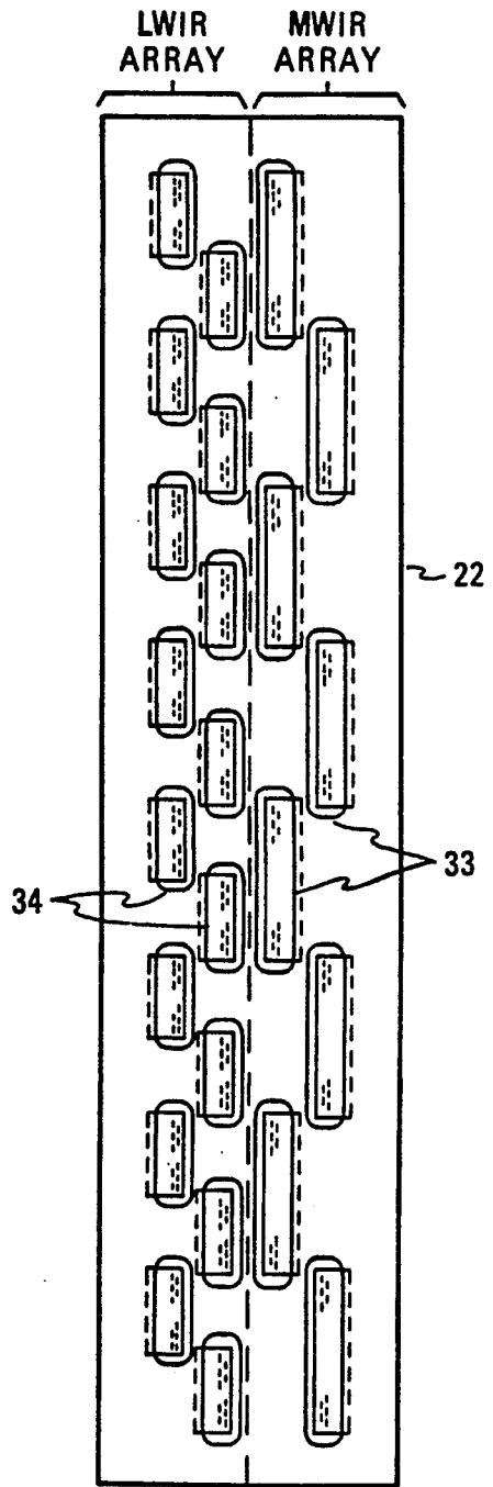
FIG. 2B "SLIT" COLD SHIELD (TOP VIEW)
