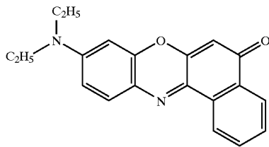
Nile red
