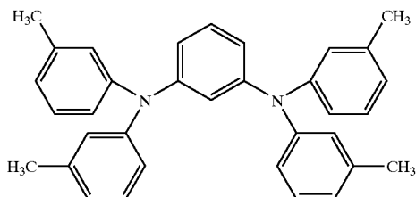
PDA
