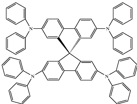
spiro-TPD
