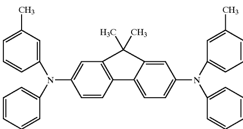
DTDPFL
