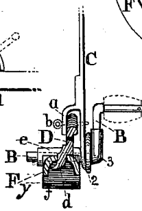
Fig. 4. (Cross-section on line "aa" Fig. 3.)
