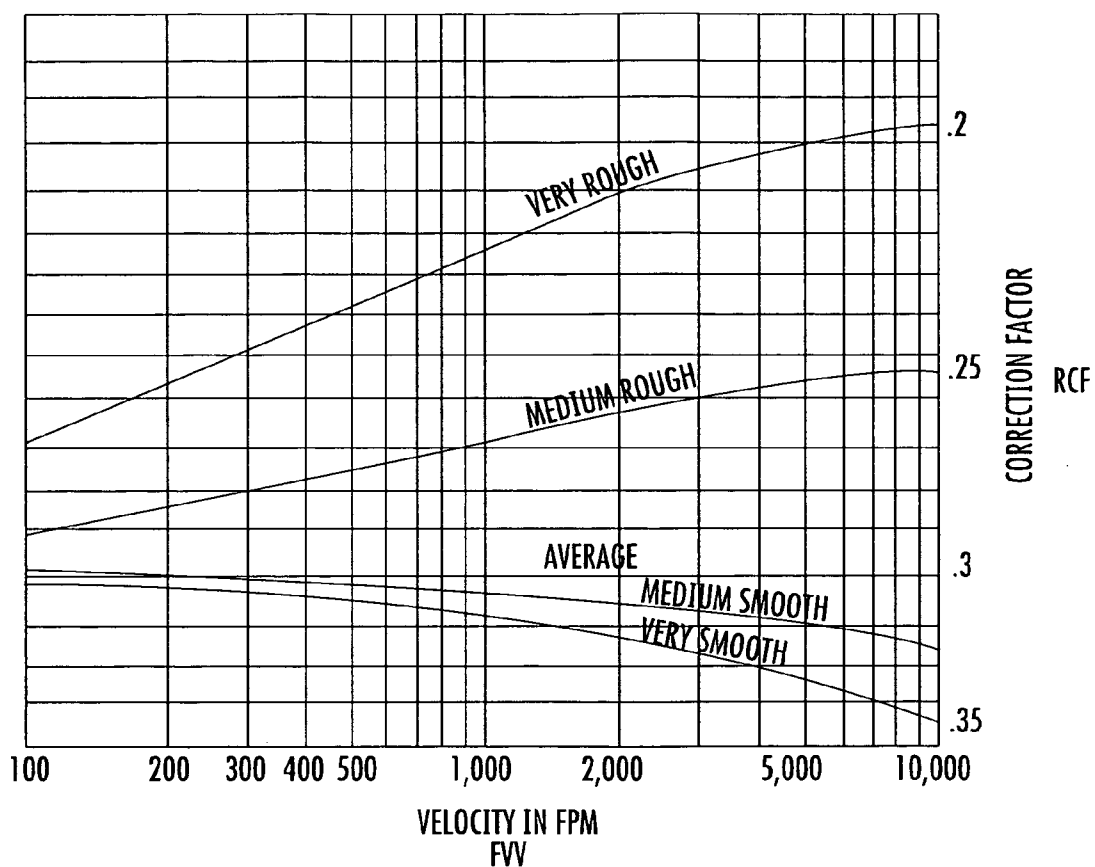
FUME HOOD LINEAR ROUGHNESS CORRECTION FACTOR (RCF)
