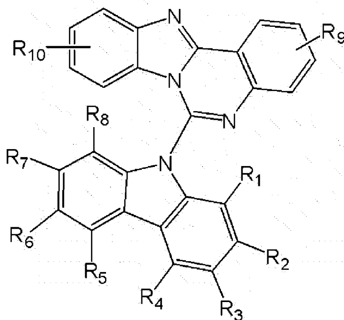
[Chemical Formula 1]
