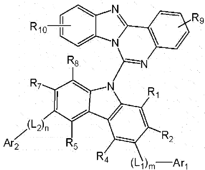
[Chemical Formula 7]
