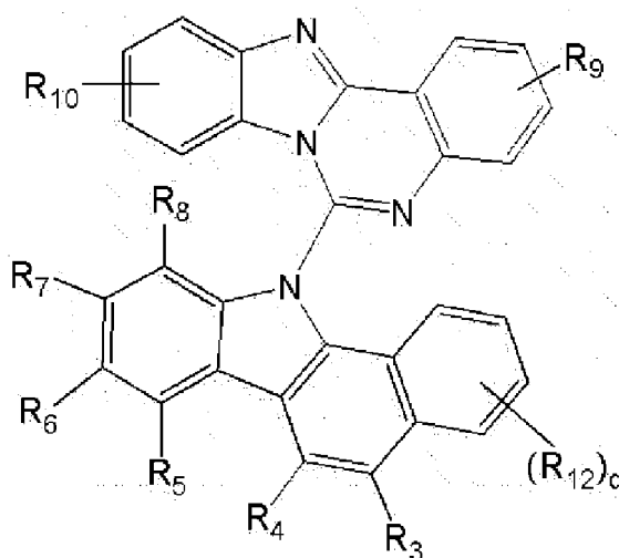
[Chemical Formula 3]
