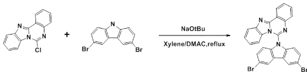
Compound C
