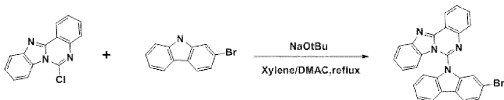
Compound B
