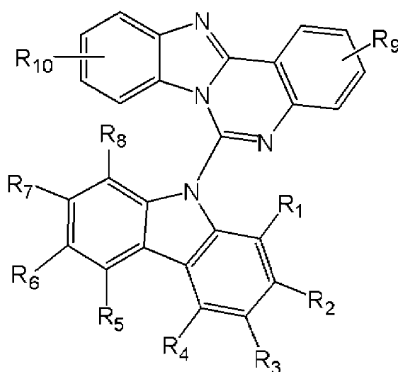
[Chemical Formula 1]
