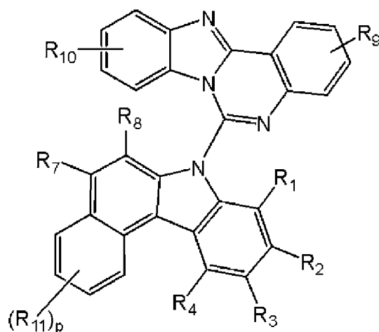
[Chemical Formula 2]
