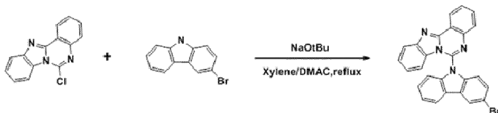
Compound A
