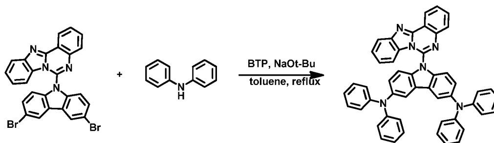
Compound 93
