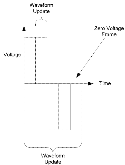
Fig. 8 (Prior Art)
