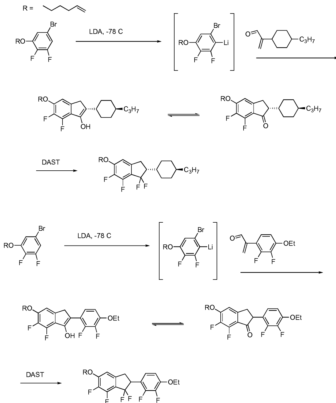
Scheme 11
