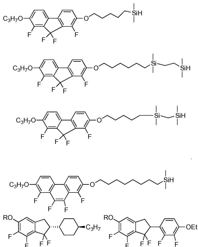
Scheme 3
