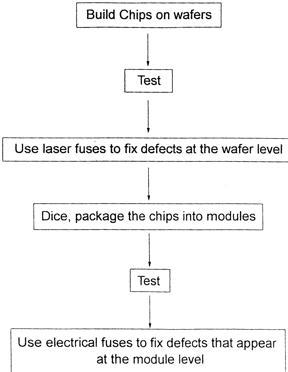
Figure1: Wafer test and repair proces flow PRIOR ART
