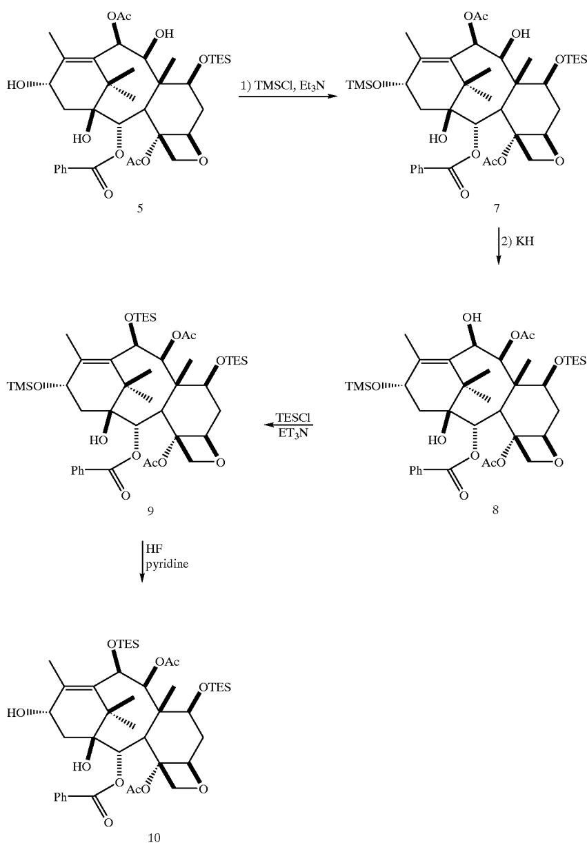
REACTION SCHEME 2
