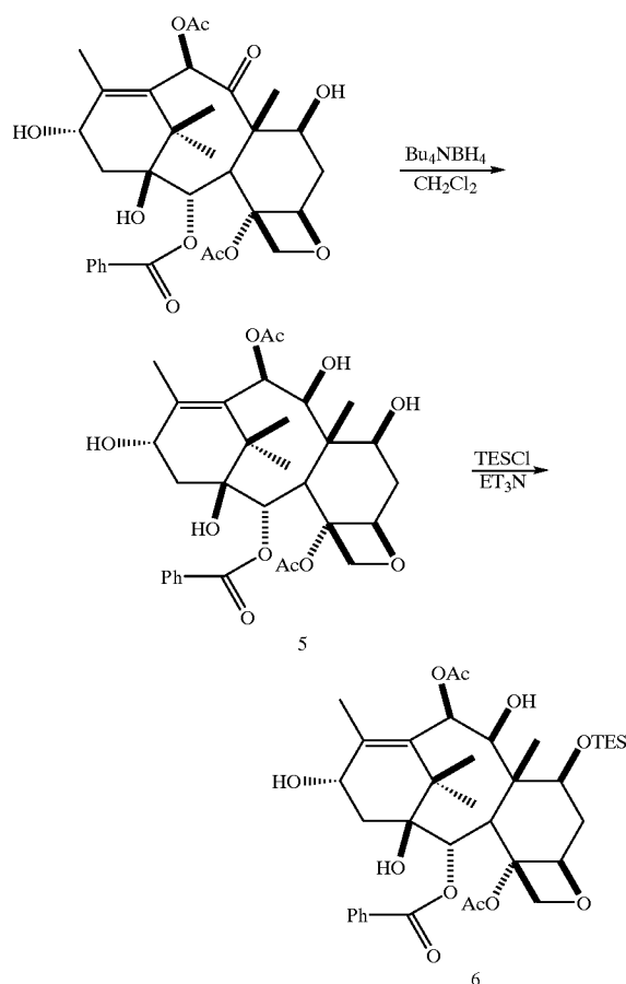
REACTION SCHEME 1
