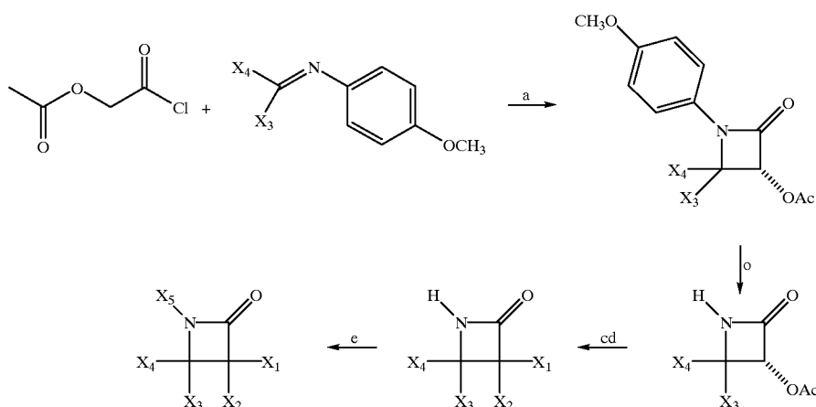
Scheme A
