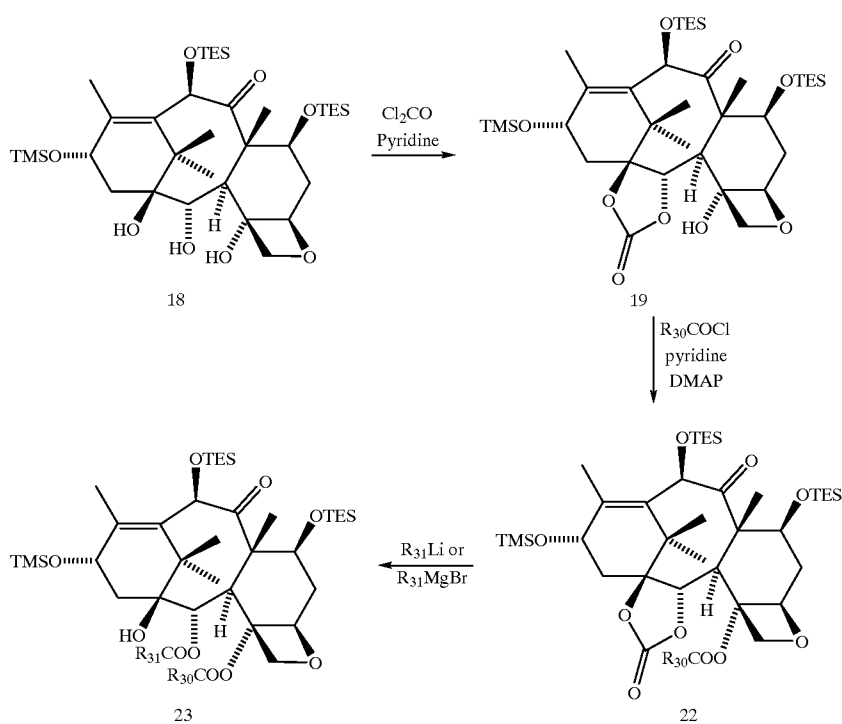
Scheme 9
