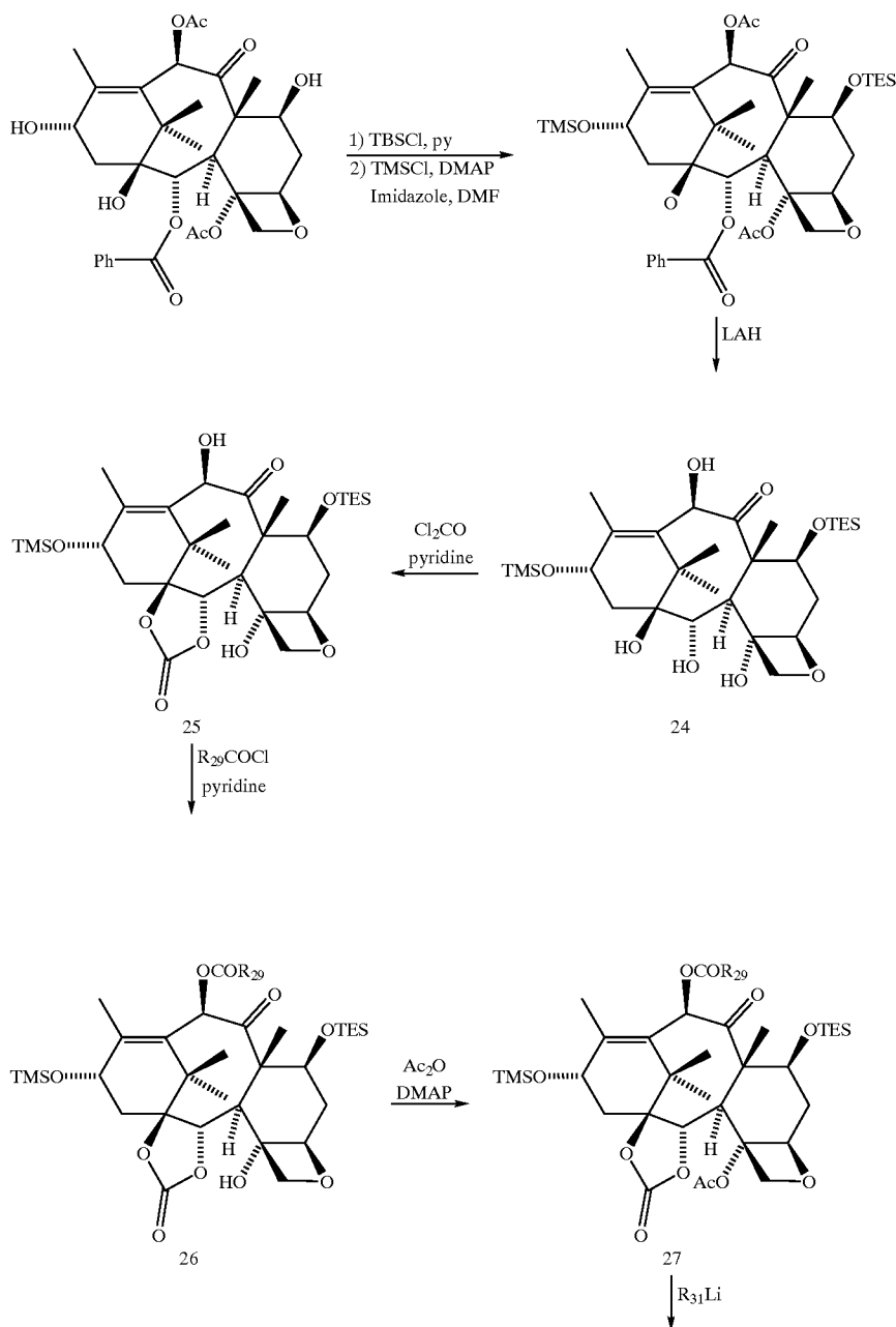
Scheme 10
