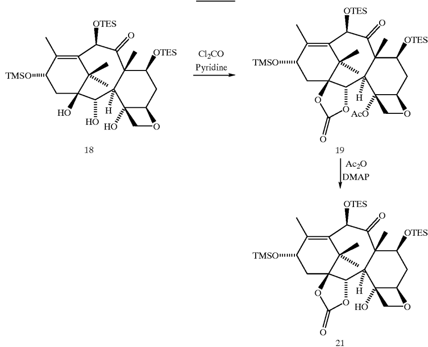
-continued Scheme 8
