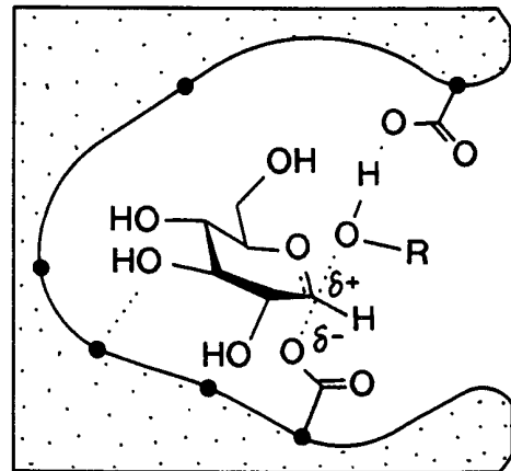
transition state binding [E-S] ‡ R = aglycon residue
