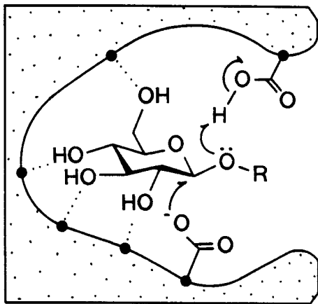
ground state binding [E-S]
