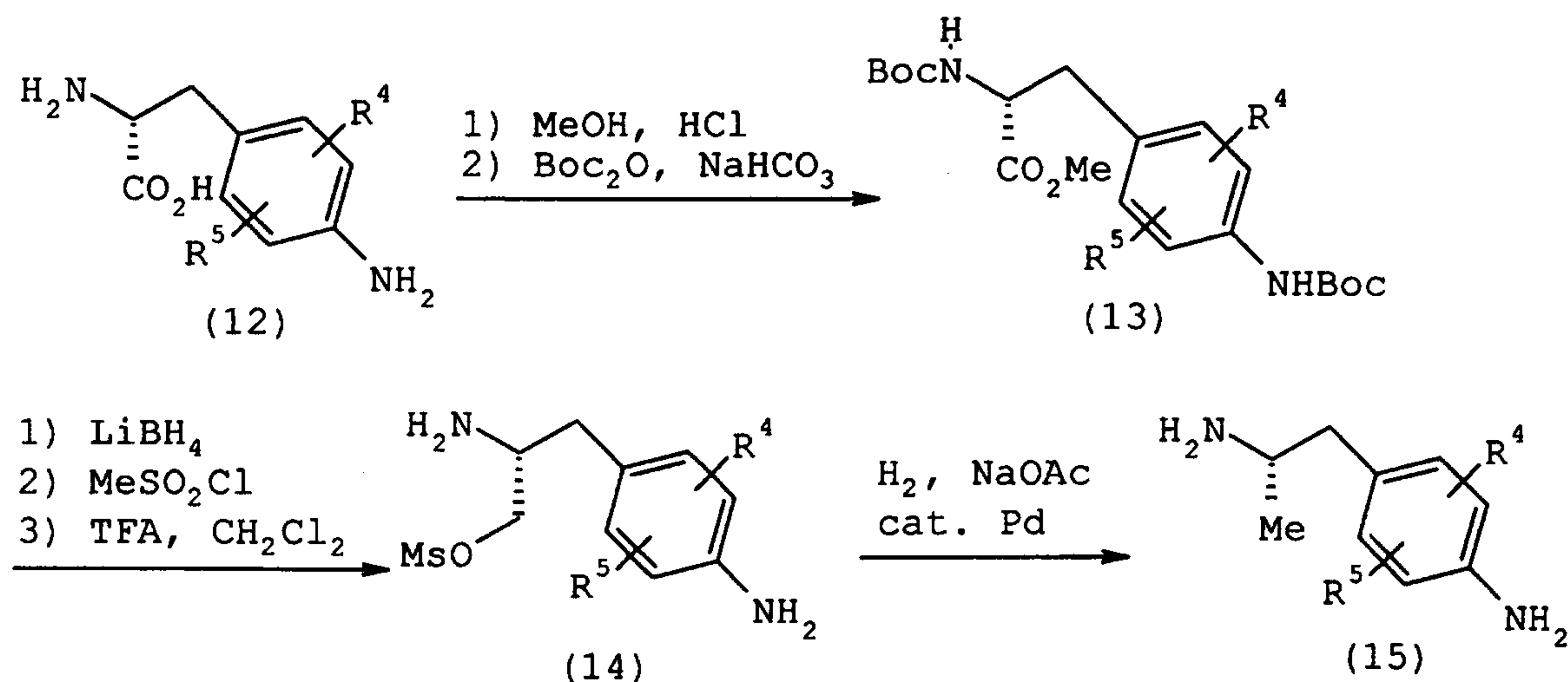
Scheme 5
