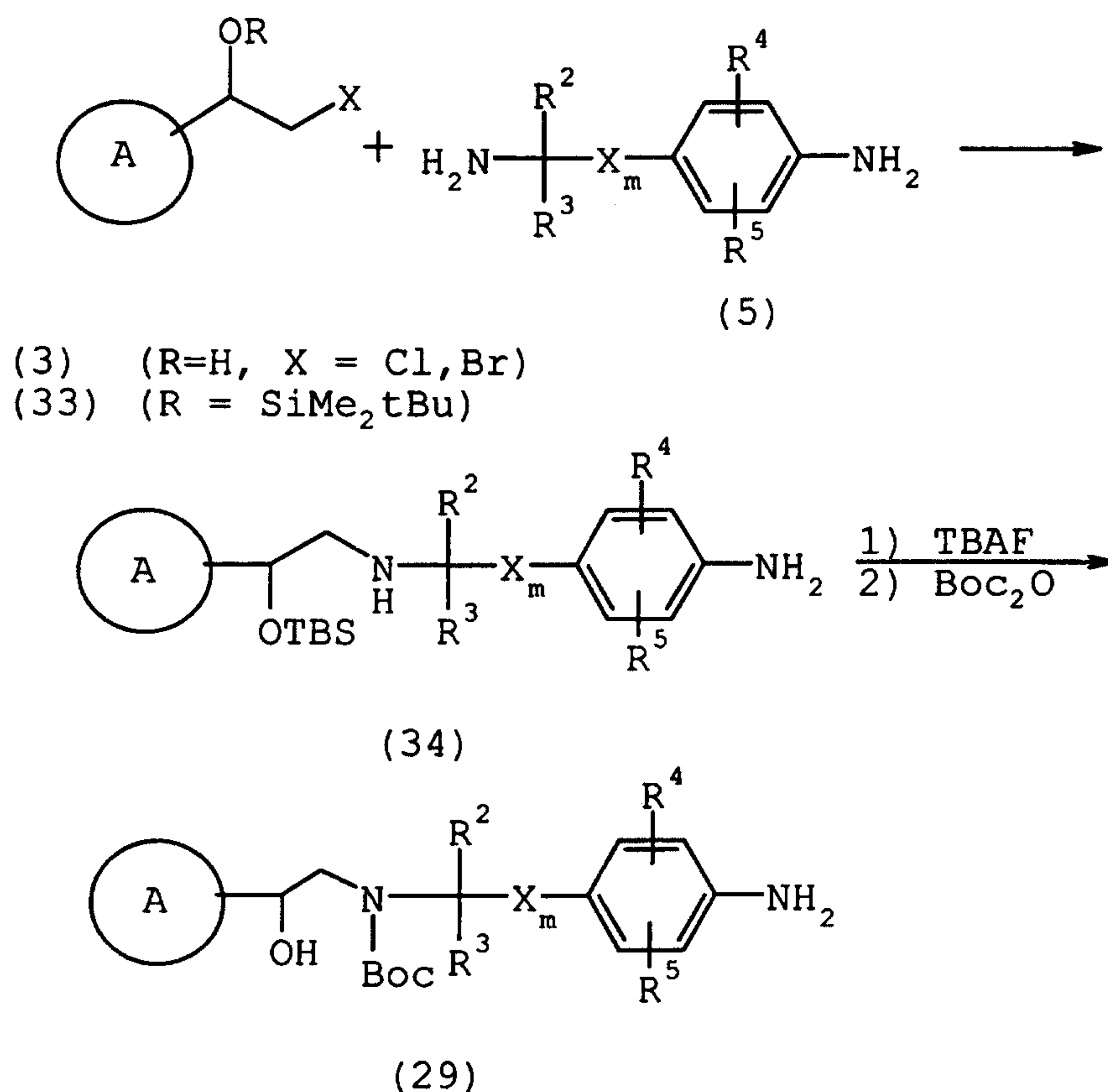
Scheme 12
