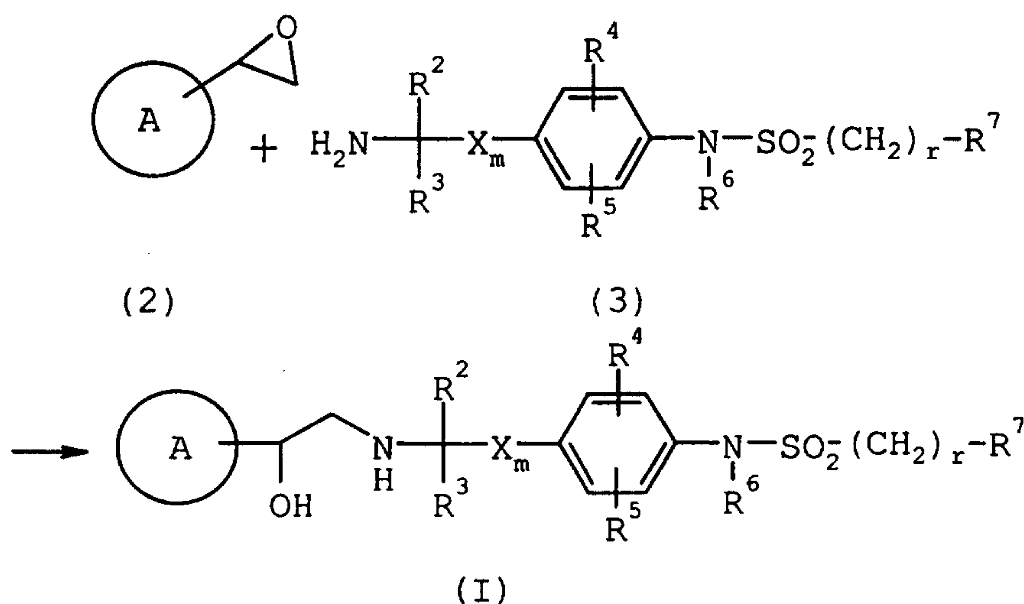
Scheme 8
