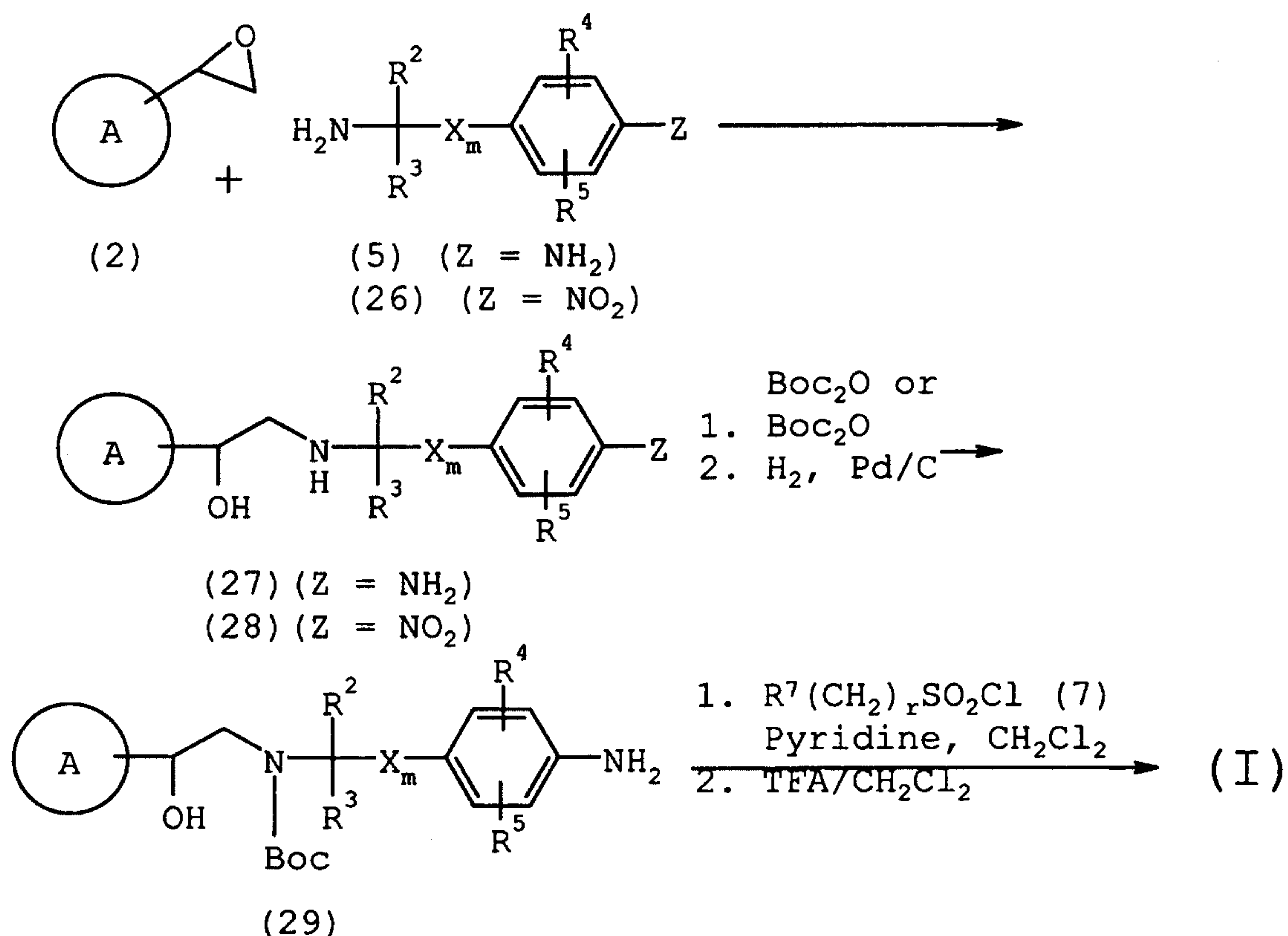
Scheme 9
