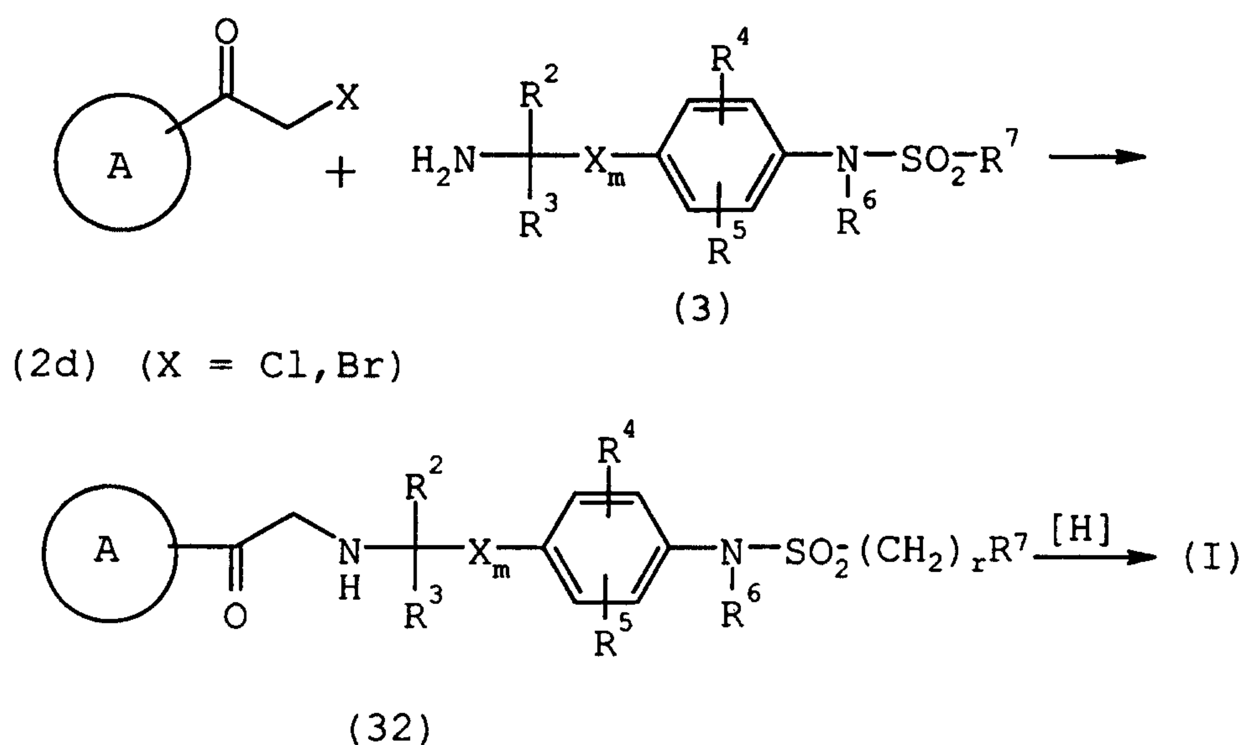
Scheme 11
