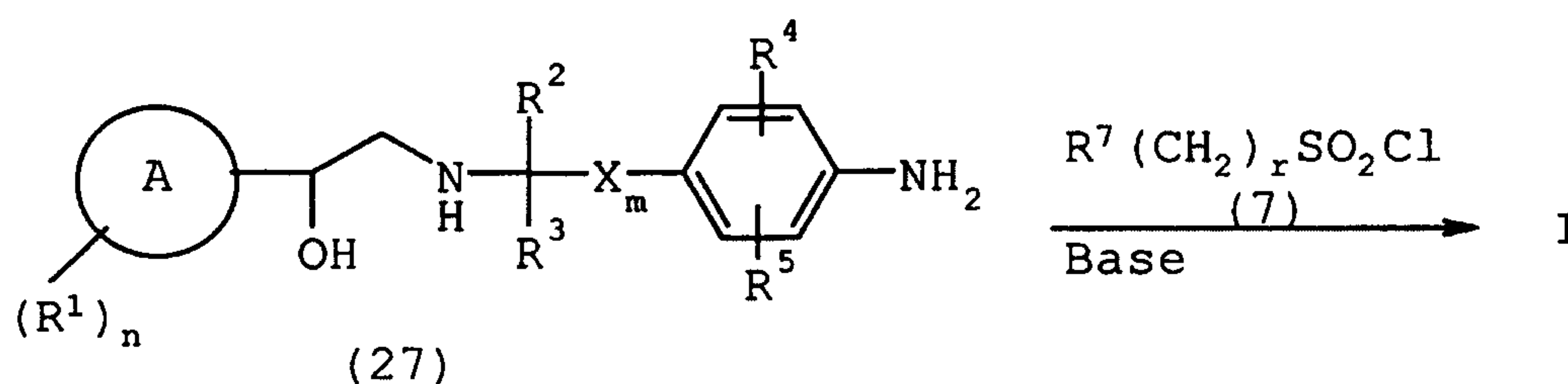
Scheme 13
