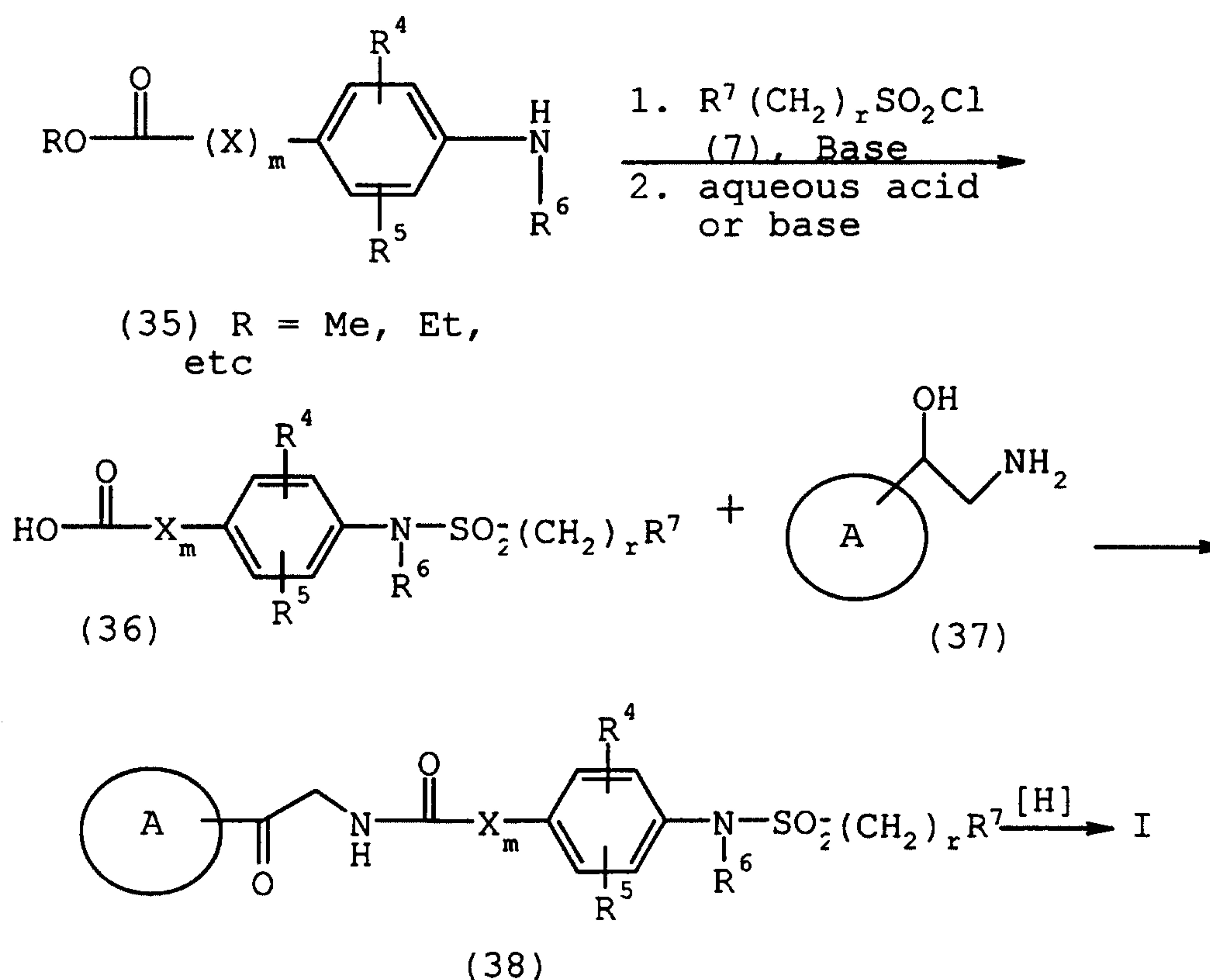
Scheme 14
