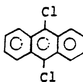
9,10-dichloroanthracene
