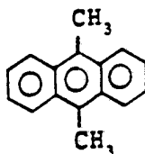
9,10-dimethylantracene
