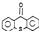
thioxanthone 2-chlorothioxanthone 1-chloroanthraquinone
