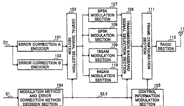
100 TRANSMITTING APPARATUS
