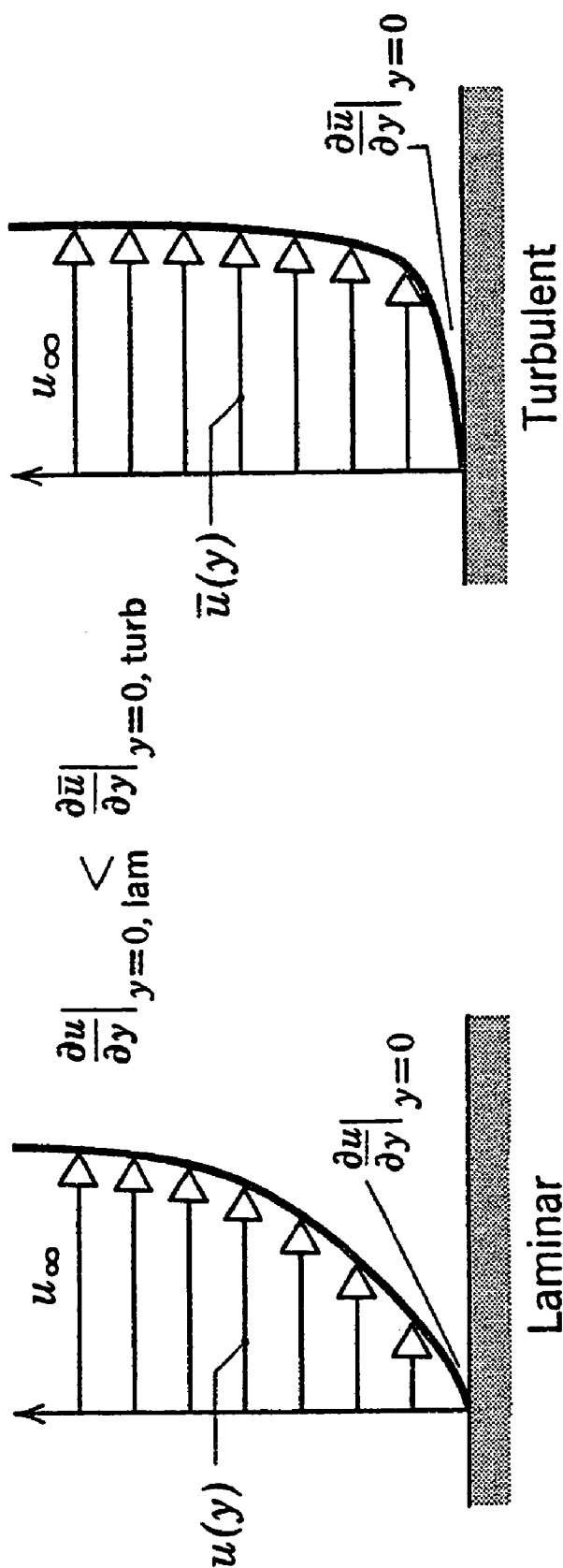
Figure 6.17 Comparison of laminar and turbulent velocity boundary layer profiles for the same freestream velocity.
