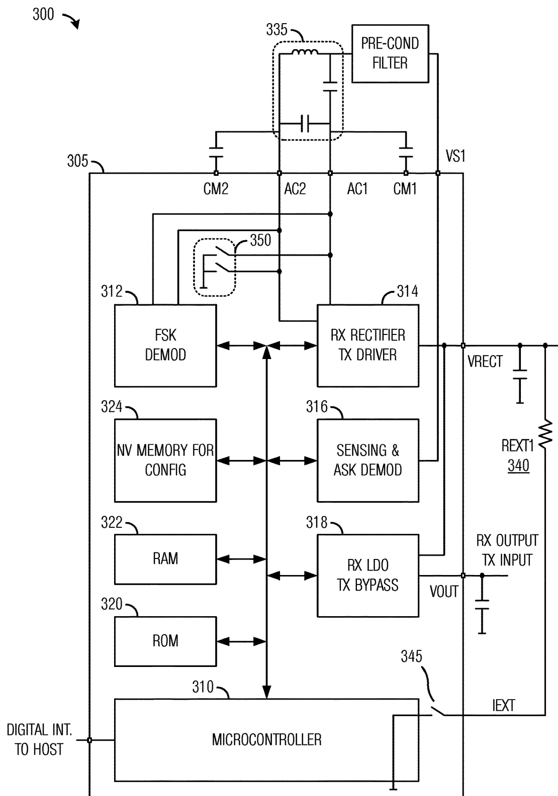
Fig. 3 (Prior Art)
