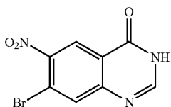
7-bromo-6-nitro-3H-quinazolin-4-one
