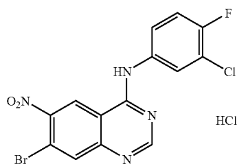
(7-bromo-6-nitro-4-quinazolinyl)-(3-chloro-4-fluorophenyl)amine hydrochloride
