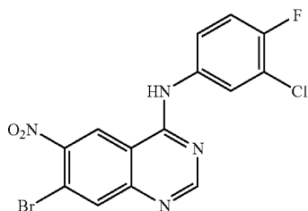
(7-bromo-6-nitro-4-quinazolinyl)-(3-chloro-4-fluorophenyl)amine
