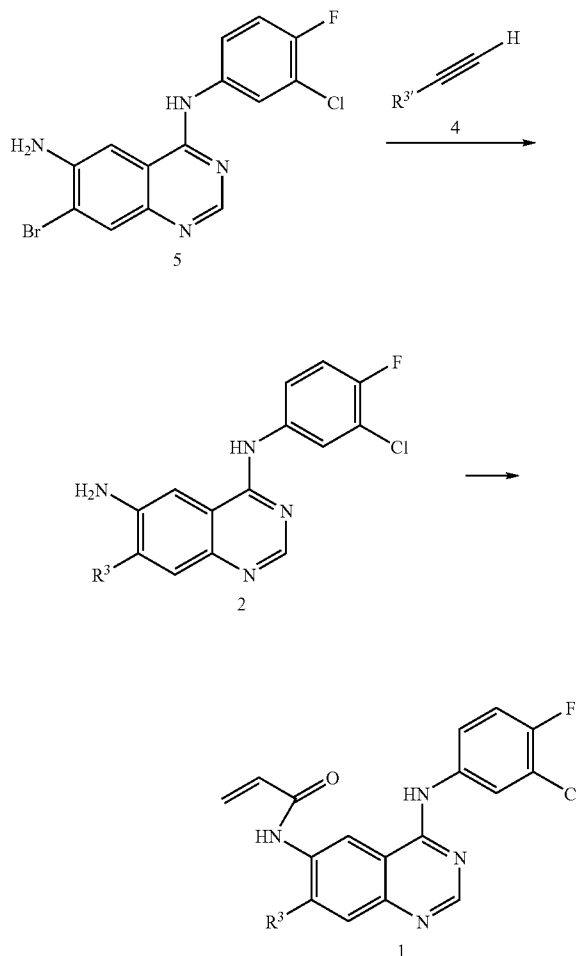
Scheme 5
