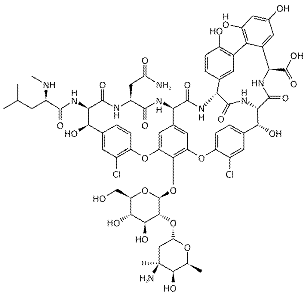
Vancomycin (Formula 1)
