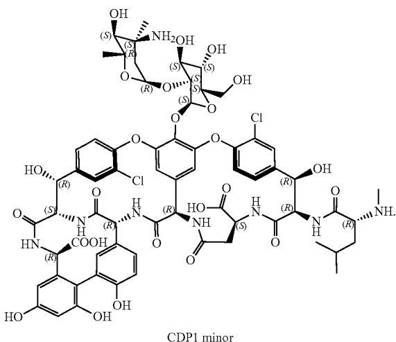
Formula 3a
