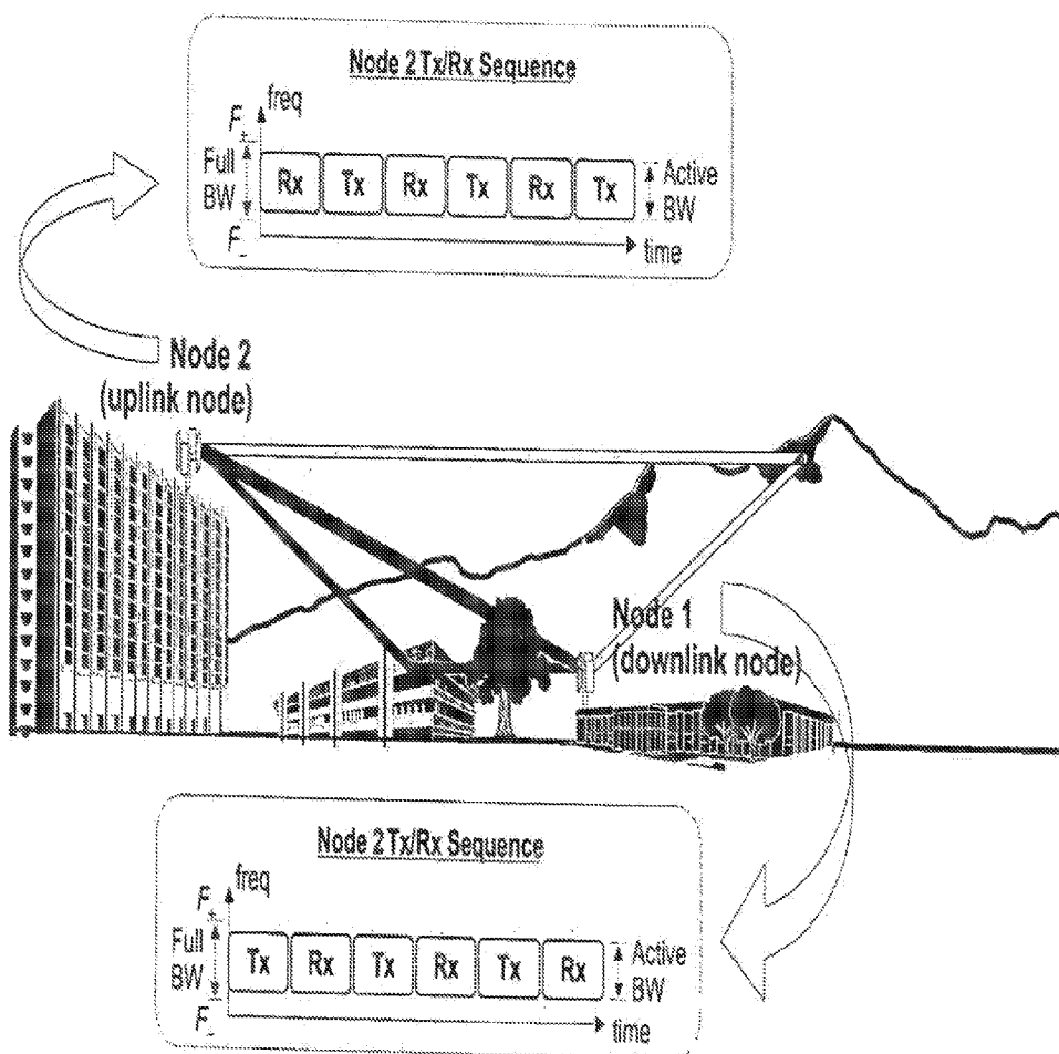
FIG. 14 Prior Art
