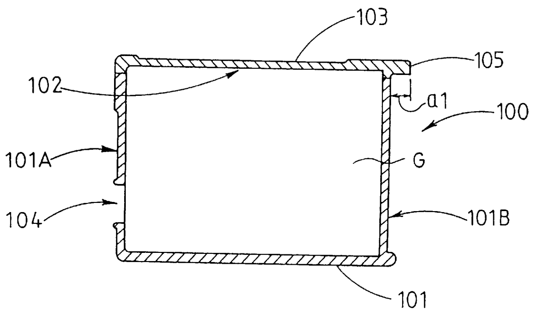
Fig.12 PRIOR ART
