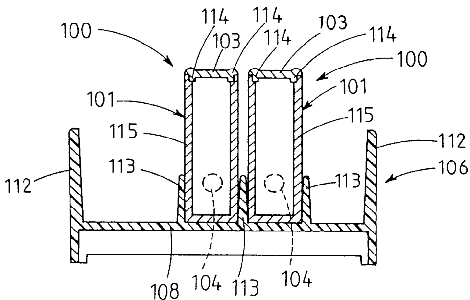
Fig.14 PRIOR ART
