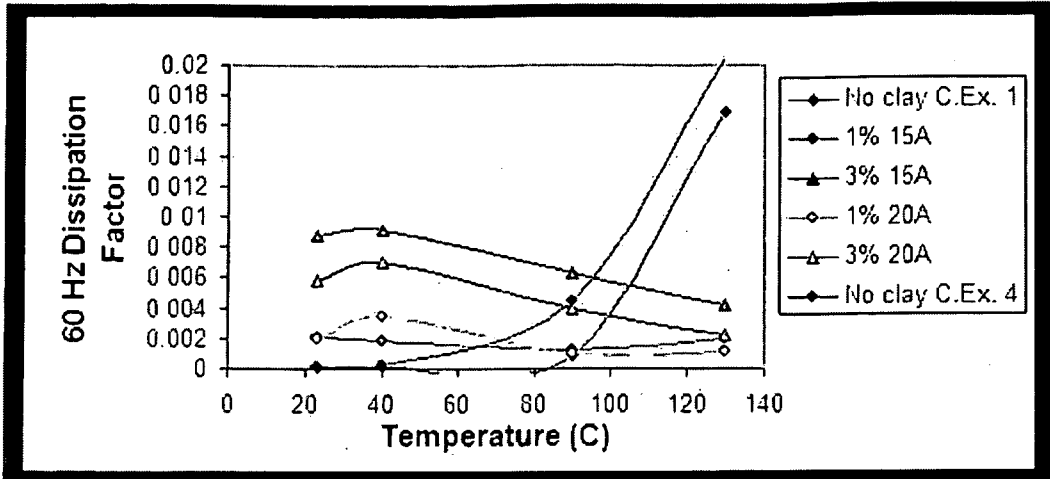
FIG 5: Graphical representation of dissipation factor data in Table 5. Comparative Examples 1 and Comparative Example 4 represent the same composition from separate preparations.
