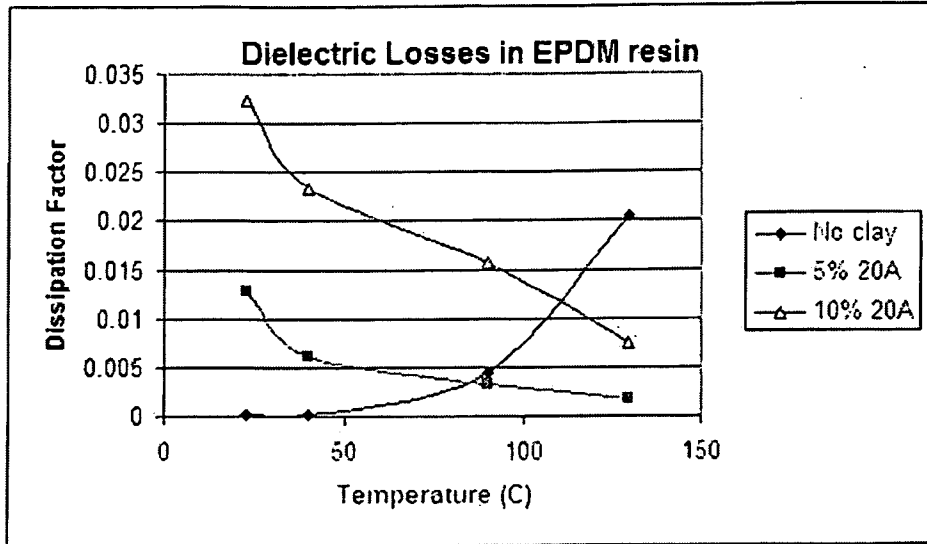
FIG 4: Graphical representation of dissipation factor data of Table 4.
