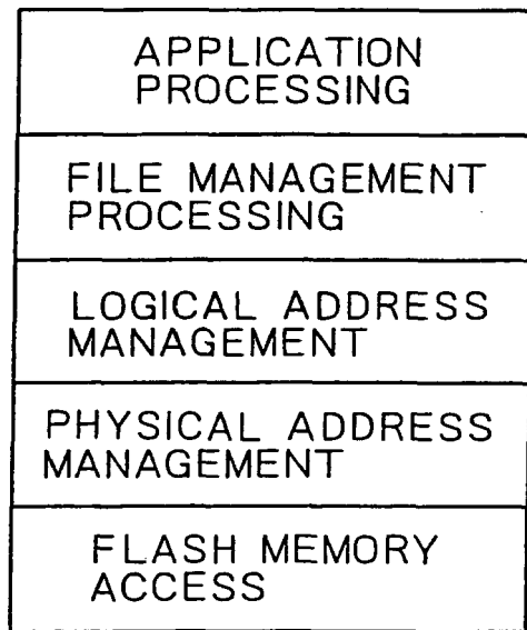
FILE SYSTEM PROCESSING HIERARCHY
