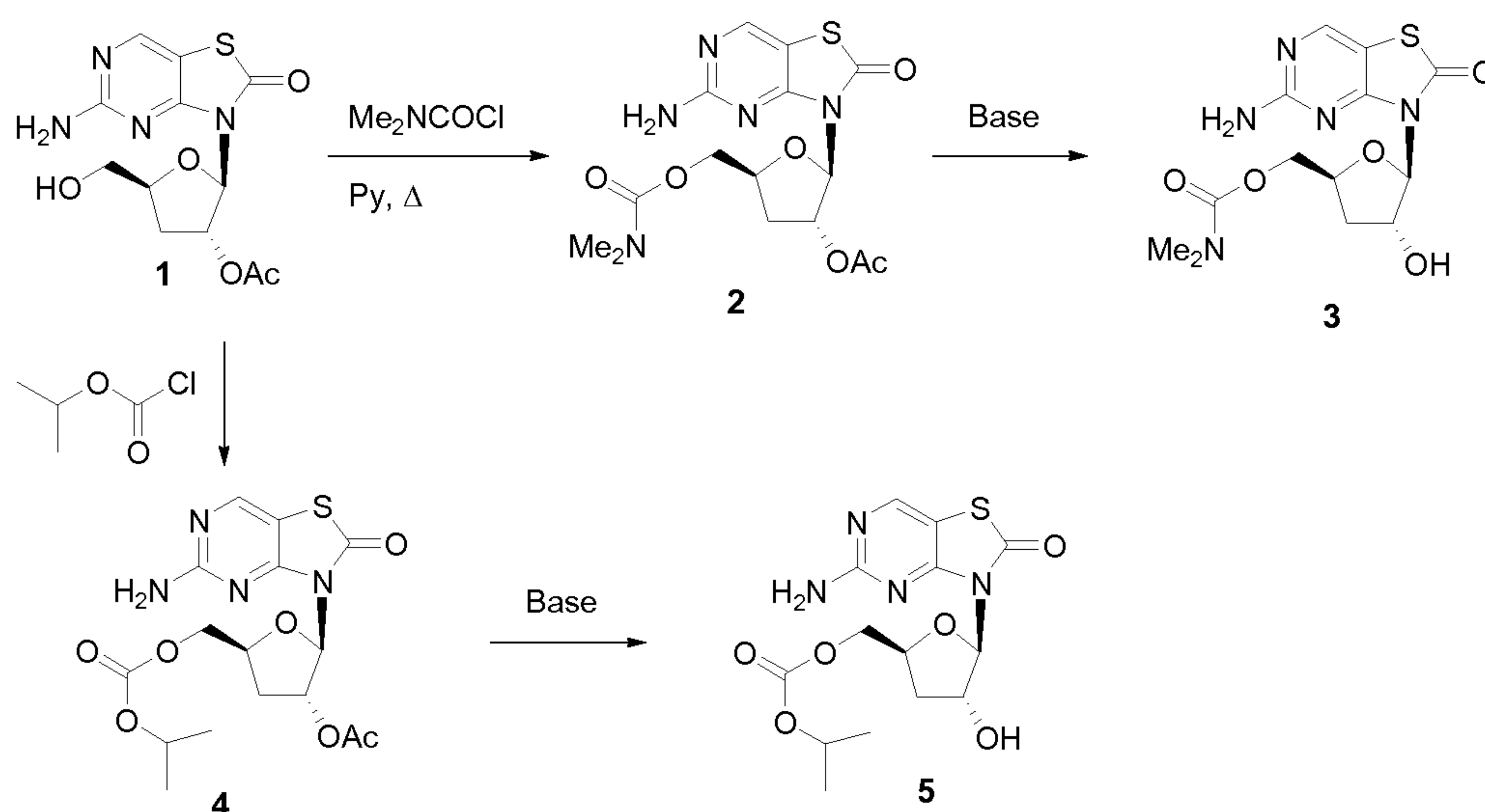
Scheme 1: 5'-Carbonates and Carbamates
