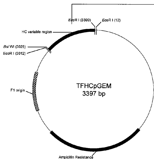
HC Cloning Vector
