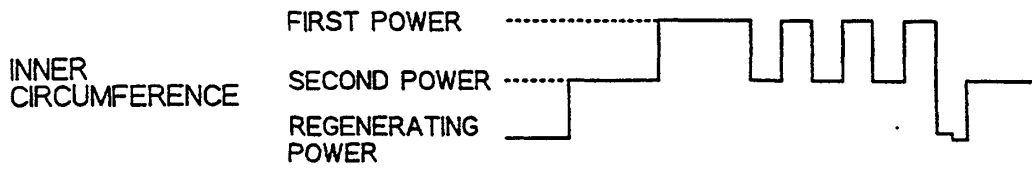
RECORDING WAVEFORM 17-2
