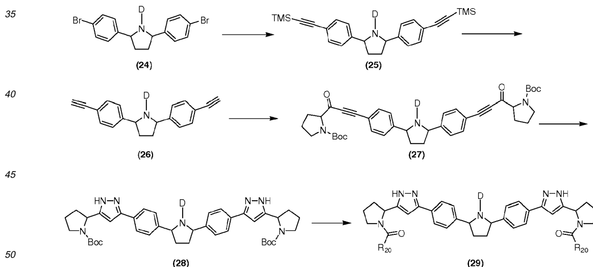
Scheme XV
