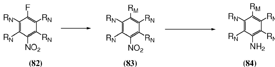
Scheme XXV
