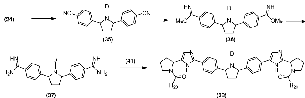
Scheme XVII
