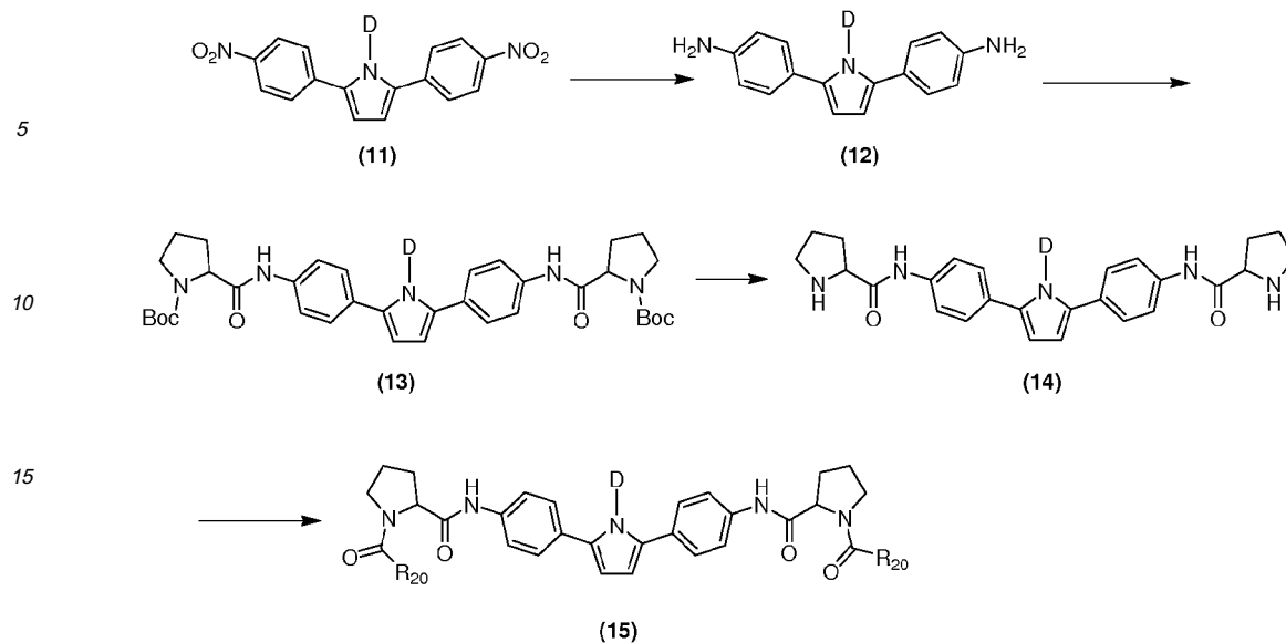
Scheme XII
