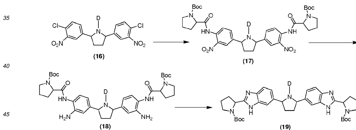
Scheme XIII
