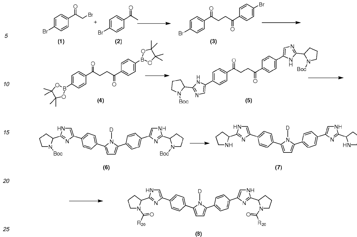
Scheme X
