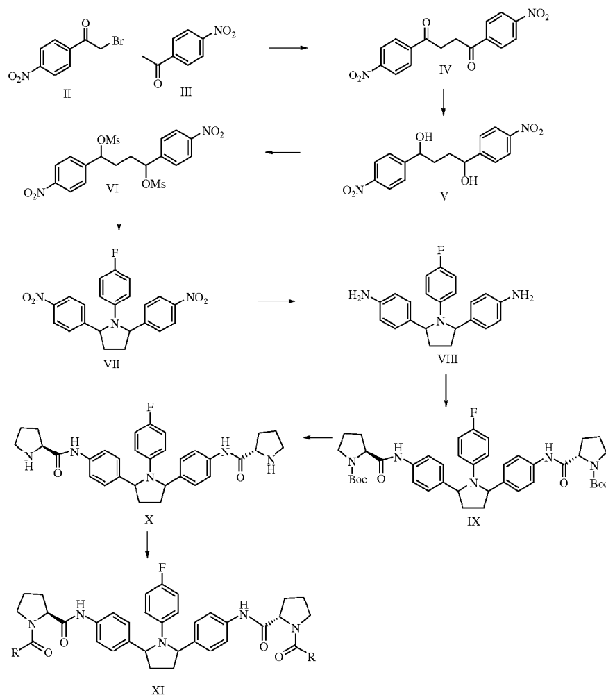
Scheme II
