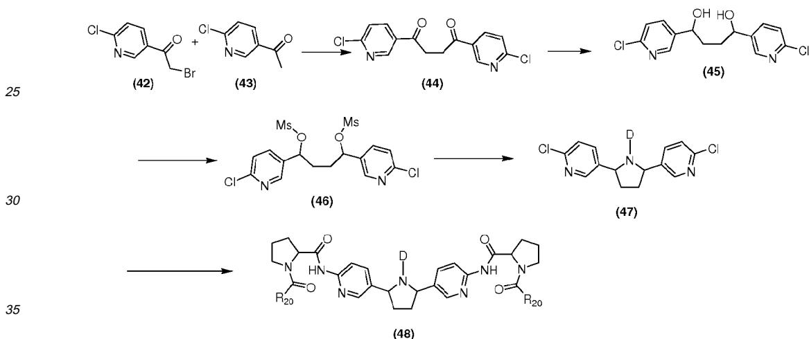
Scheme XIX
