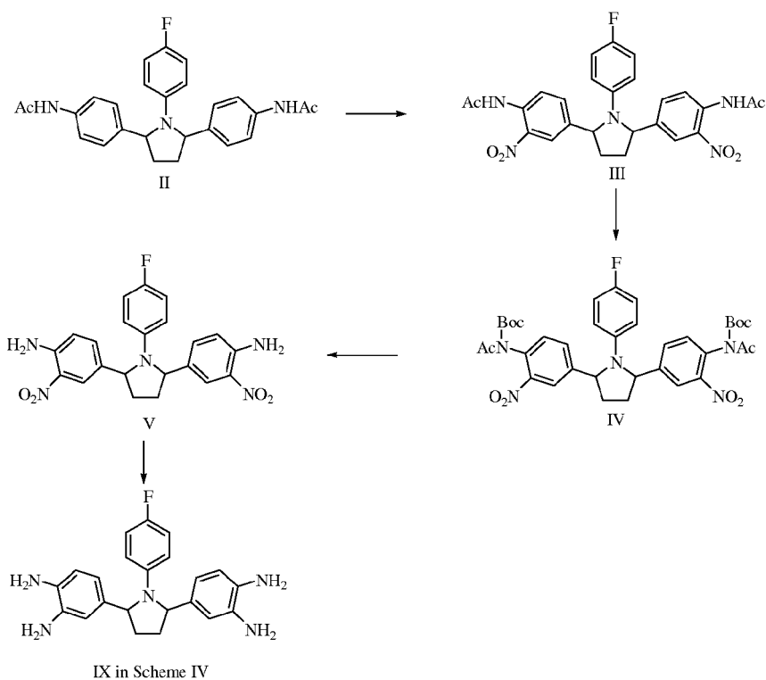
Scheme V
