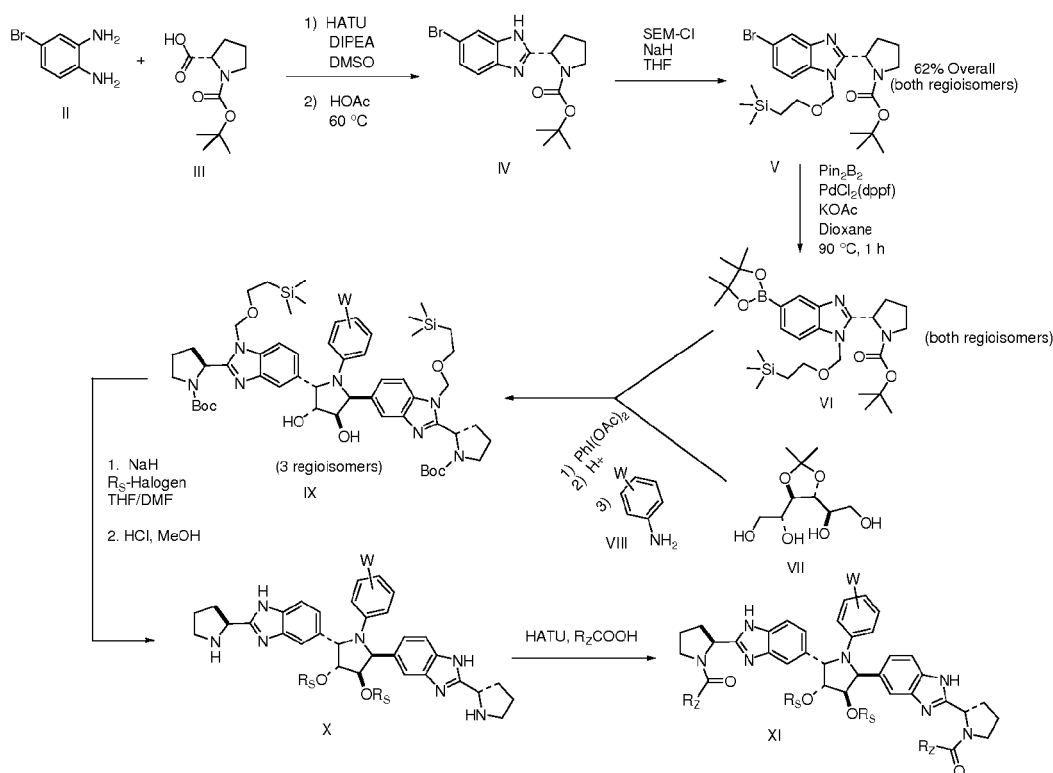
Scheme IX
