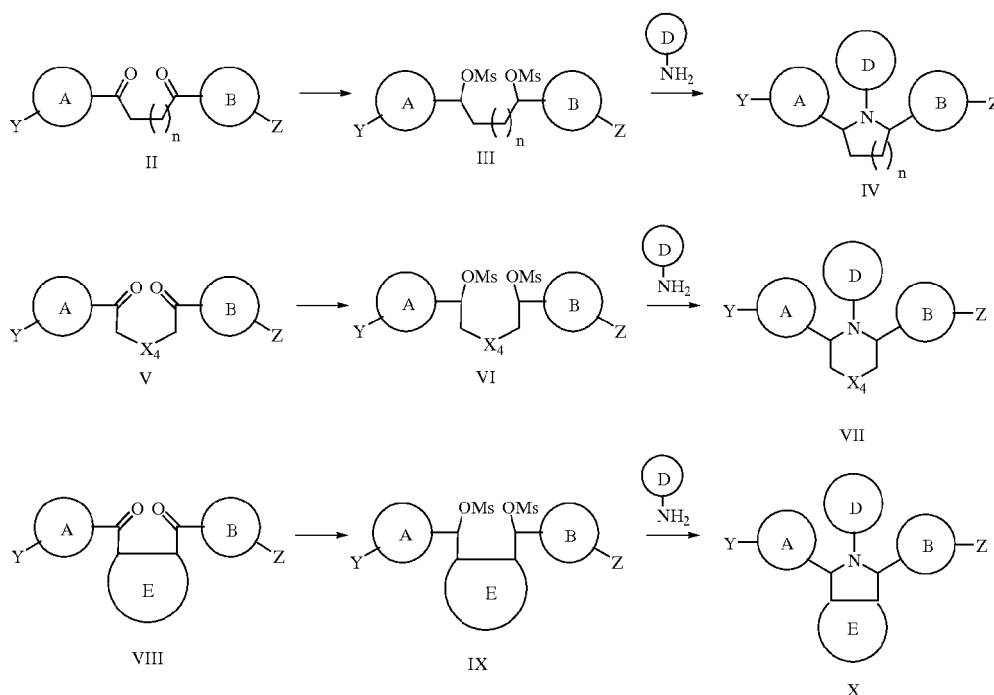
Scheme I
