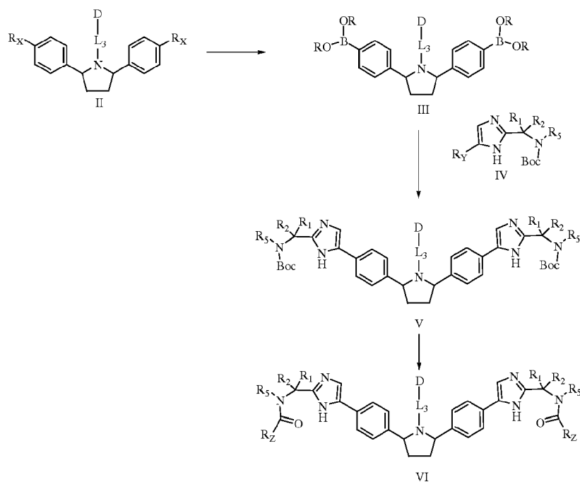
Scheme VII
