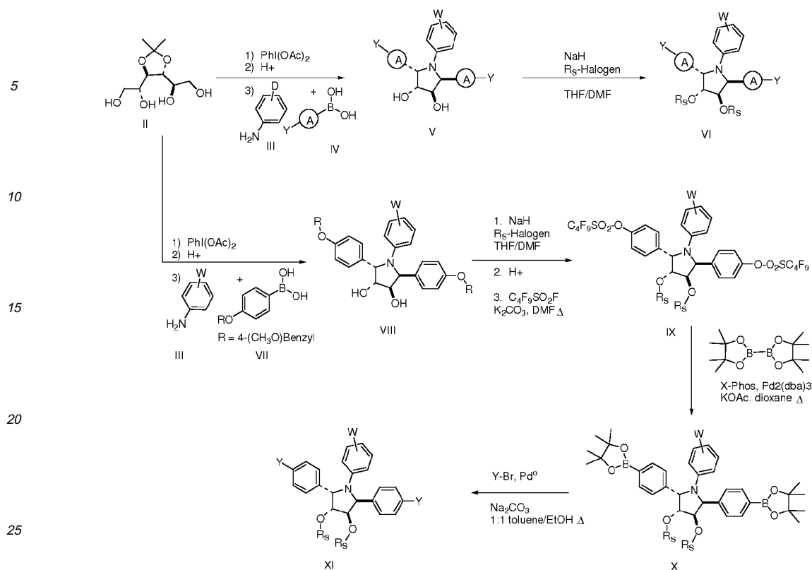
Scheme VIII
