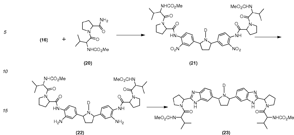
Scheme XIV
