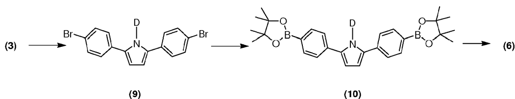
Scheme XI
