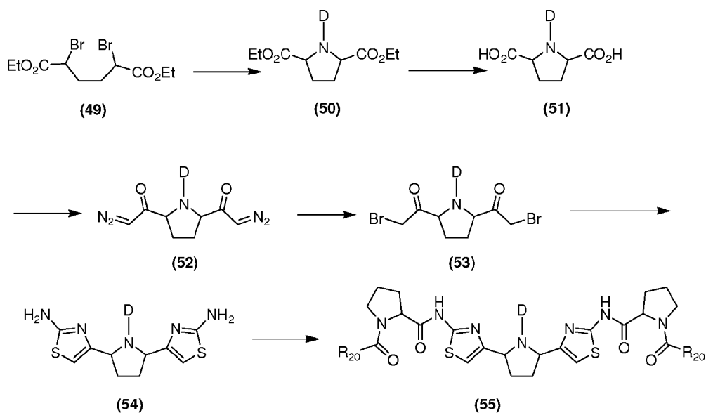
Scheme XX
