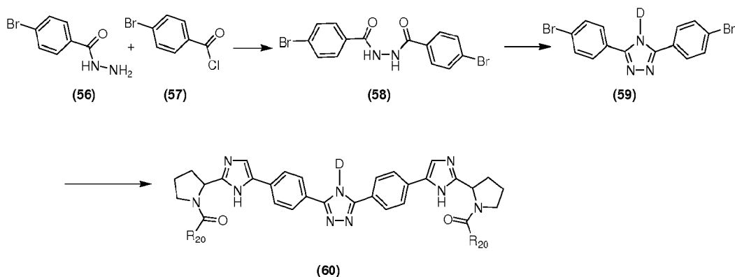
Scheme XXI
