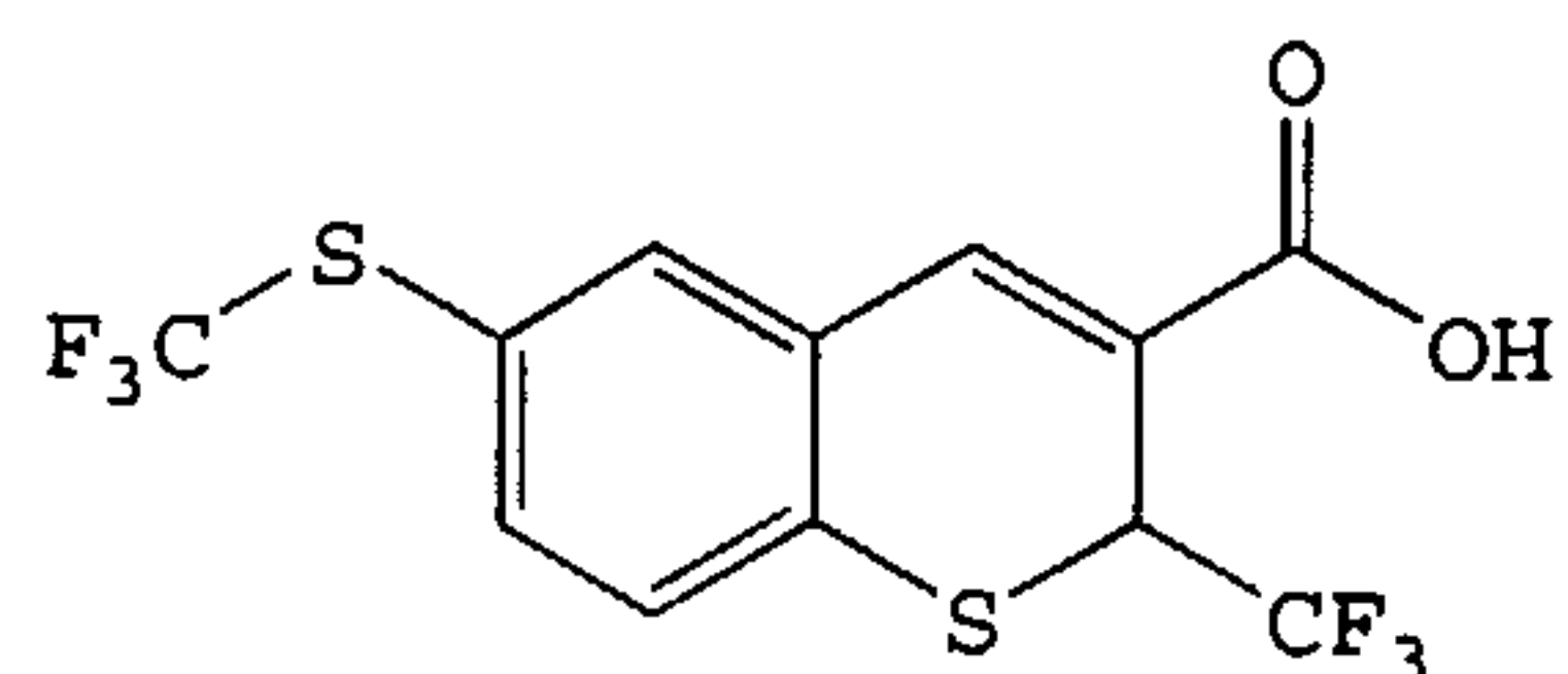
2-(Trifluoromethyl)-6-[(trifluoromethyl)thio] -2H-1-benzothiopyran-3-carboxylic acid
