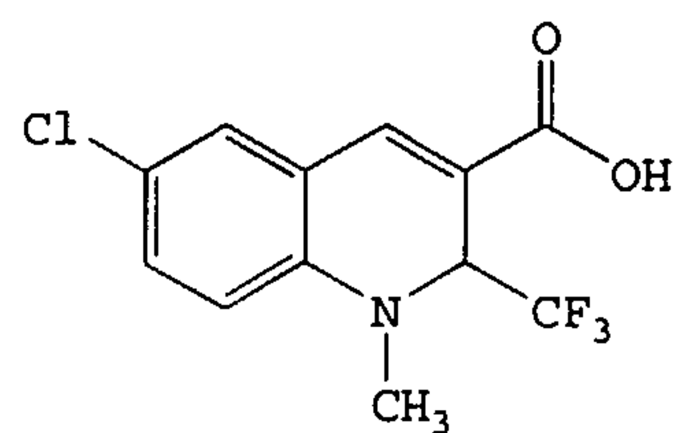
6-Chloro-1,2-dihydro-1-methyl-2-(trifluoromethyl)-3-quinolinecarboxylic acid
