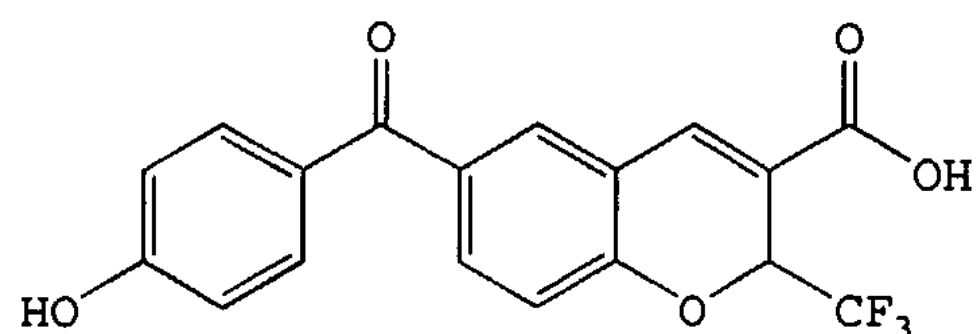
6-(4-Hydroxybenzoyl)-2-(trifluoromethyl)-2H-1-benzopyran-3-carboxylic acid
