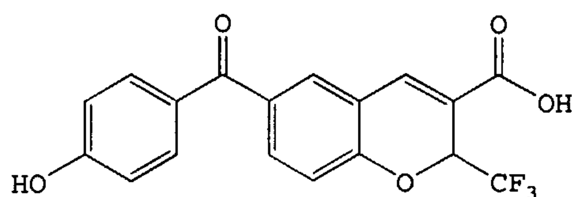
6-(4-Hydroxybenzoyl)-2-(trifluoromethyl)- 2H-1-benzopyran-3-carboxylic acid
