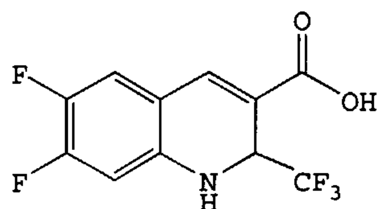
6,7-Difluoro-1,2-dihydro-2-(trifluoromethyl)-3-quinolinecarboxylic acid
