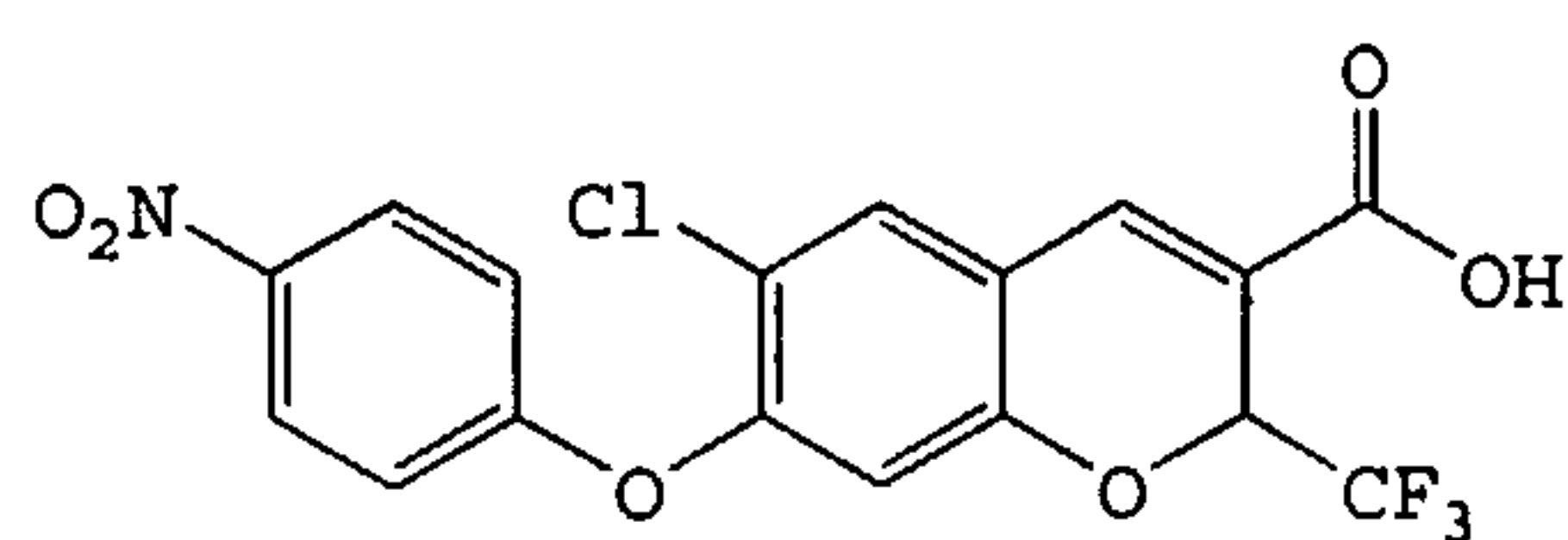
6-Chloro-7-(4-nitrophenoxy)-2-(trifluoromethyl)-2H-1- benzopyran-3-carboxylic acid
