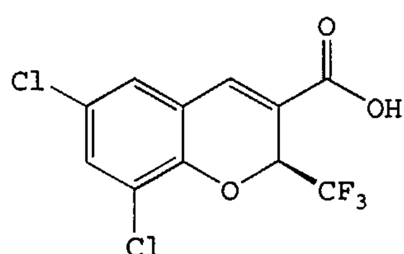
((S)-6,8-Dichloro-2-(trifluoromethyl)-2H-1-benzopyran-3-carboxylic acid
