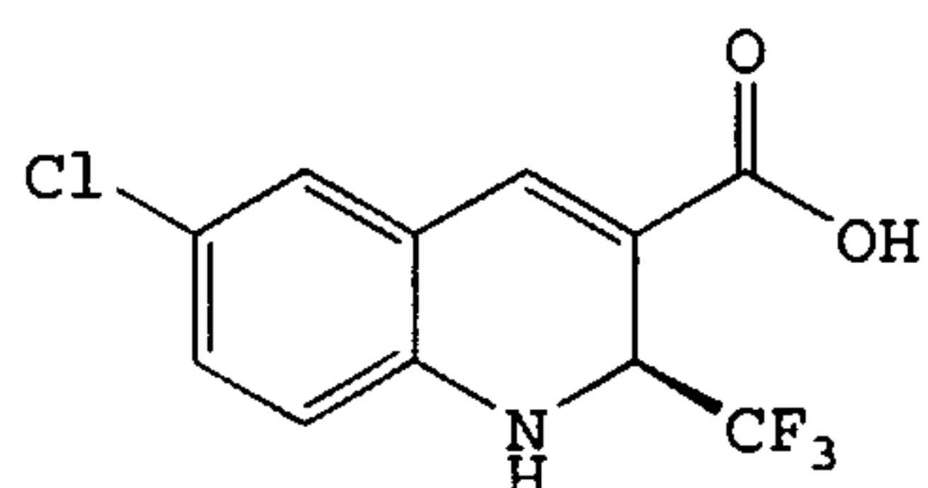
((S)-6-Chloro-1,2-dihydro-2-(trifluoromethyl)-3-quinolinecarboxylic acid
