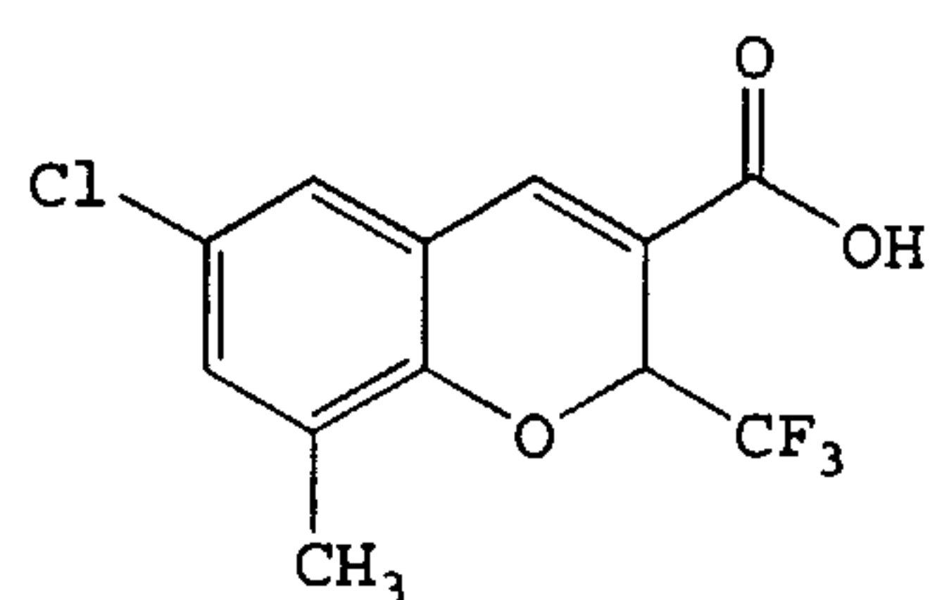
6-Chloro-8-methyl-2-trifluoromethyl- -2H-1-benzopyran-3-carboxylic acid
