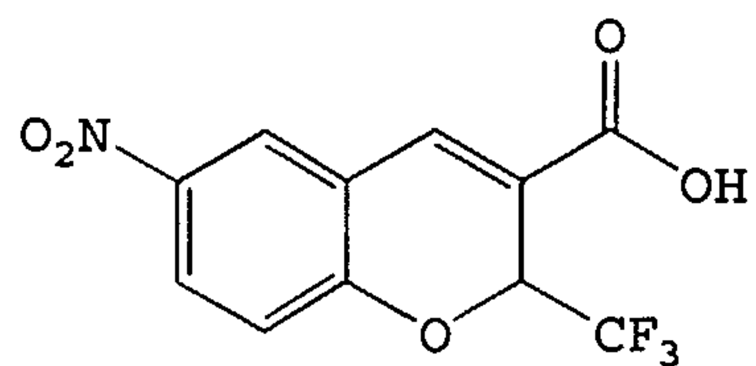
6-Nitro-2-trifluoromethyl-2H-1-benzopyran-3-carboxylic acid
