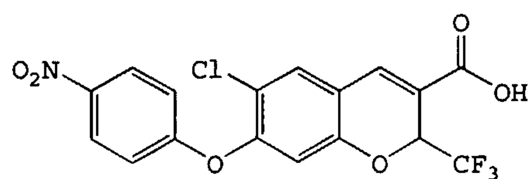
6-Chloro-7-(4-nitrophenoxy)-2-(trifluoromethyl)-2H-1-benzopyran-3-carboxylic acid
