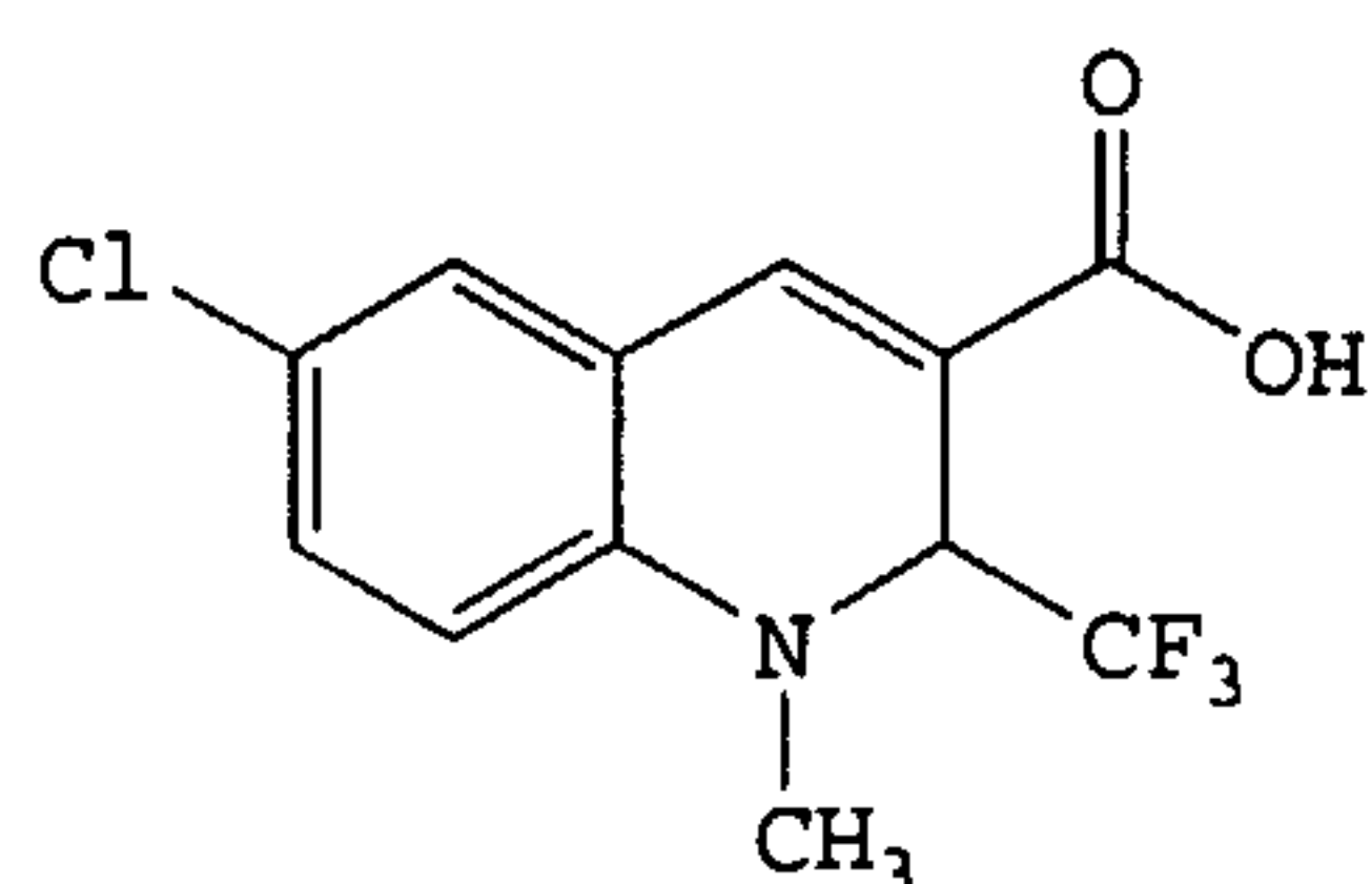
6-Chloro-1,2-dihydro-1-methyl-2-(trifluoromethyl)-3-quinolinecarboxylic acid
