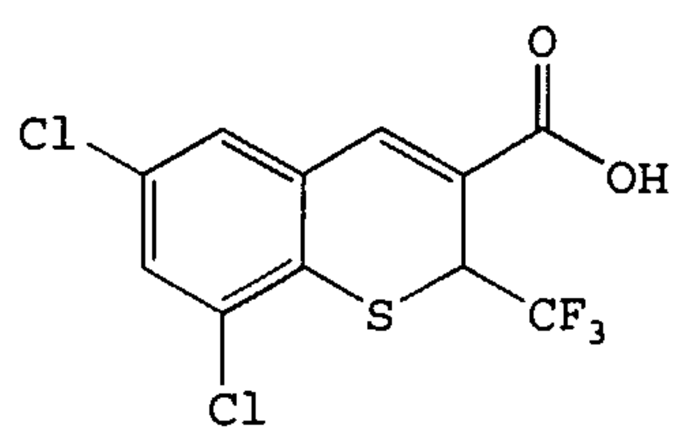
6,8-Dichloro-2-(trifluoromethyl)-2H-1-benzothiopyran-3-carboxylic acid
