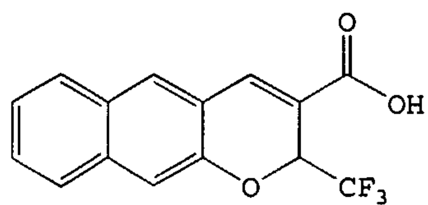
2-Trifluoromethyl-2H-naphtho[2,3-b]pyran-3-carboxylic acid
