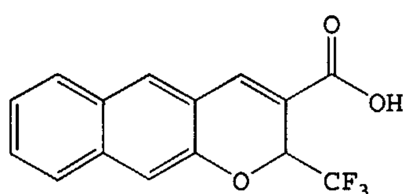
2-Trifluoromethyl-2H-naphtho[2,3-b] pyran-3-carboxylic acid
