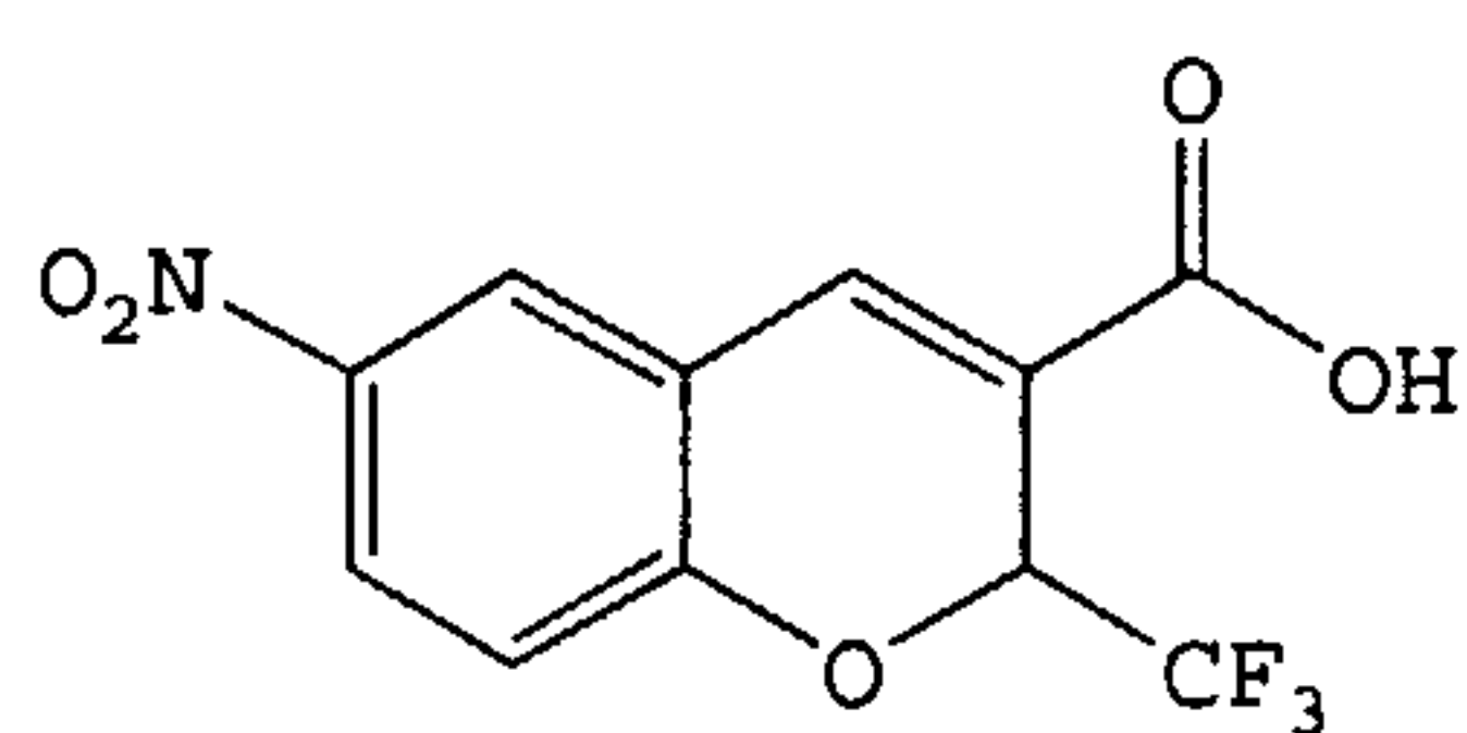
6-Nitro-2-trifluoromethyl-2H-1-benzopyran-3-carboxylic acid
