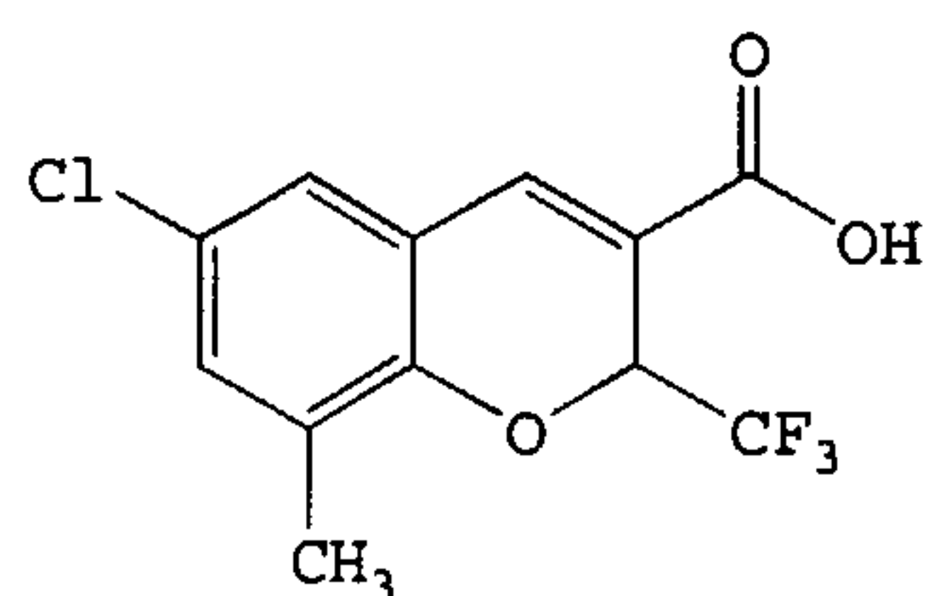
6-Chloro-8-methyl-2-trifluoromethyl-2H-1-benzopyran-3-carboxylic acid
