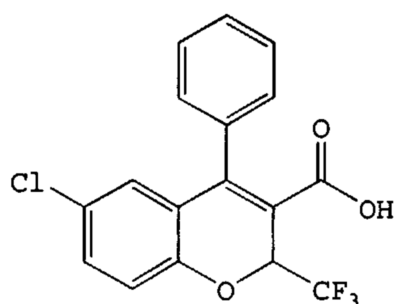
6-Chloro-2-(trifluoromethyl)-4-phenyl-2H-1-benzopyran-3-carboxylic acid
