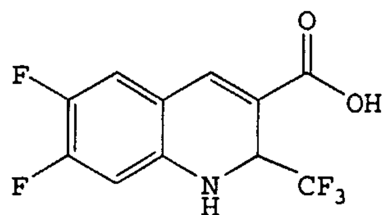
6,7-Difluoro-1,2-dihydro-2-(trifluoro methyl)-3-quinolinecarboxylic acid
