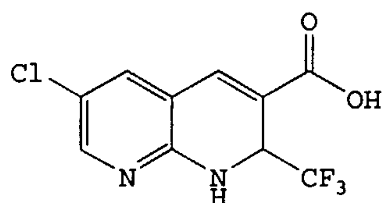
6-Chloro-2-(trifluoromethyl)-1,2-dihydro[1,8]naphthyridine-3-carboxylic acid
