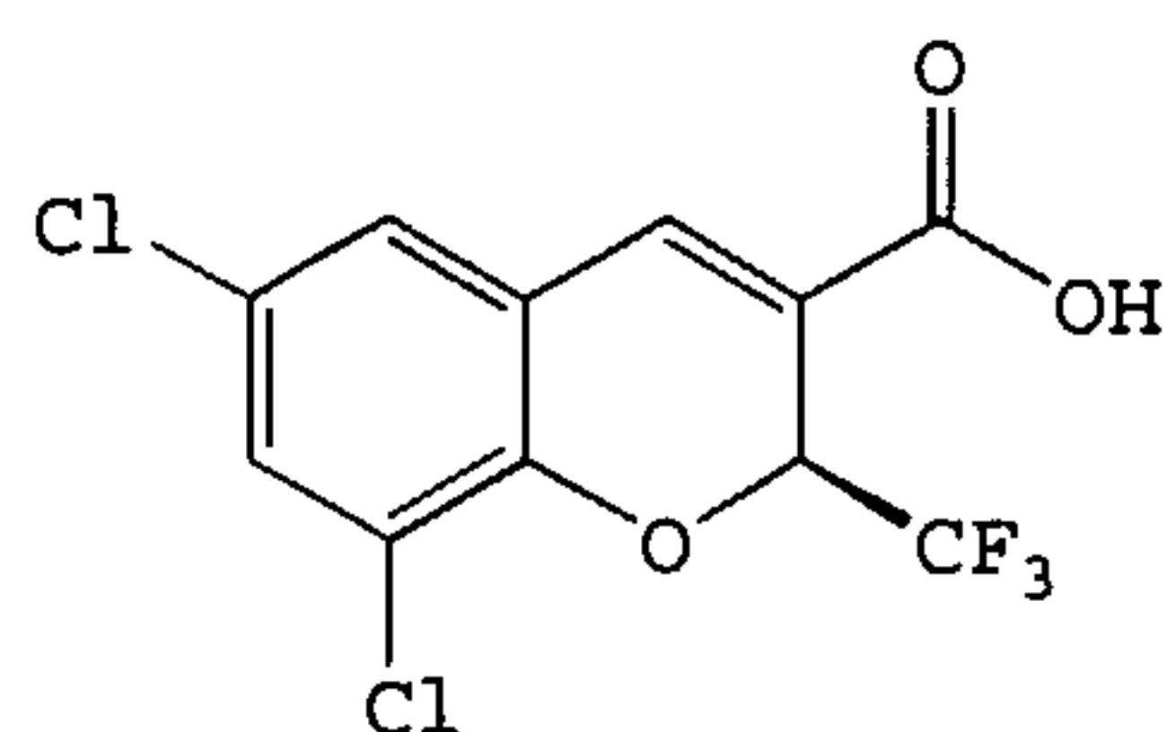
((S)-6,8-Dichloro-2-(trifluoromethyl)- 2H-1-benzopyran-3-carboxylic acid
