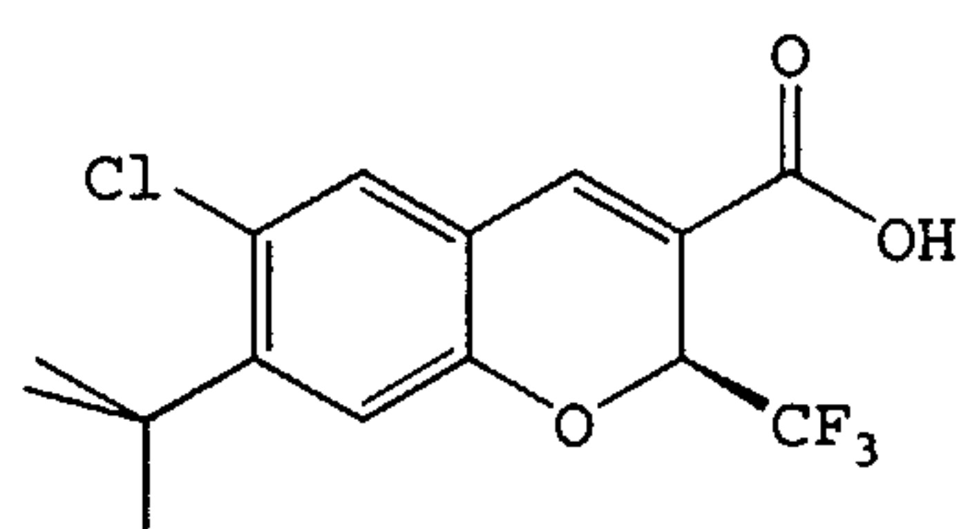
((S)-6-Chloro-7-(1,1-dimethylethyl)-2-(trifluo- romethyl-2H-1-benzopyran-3-carboxylic acid
