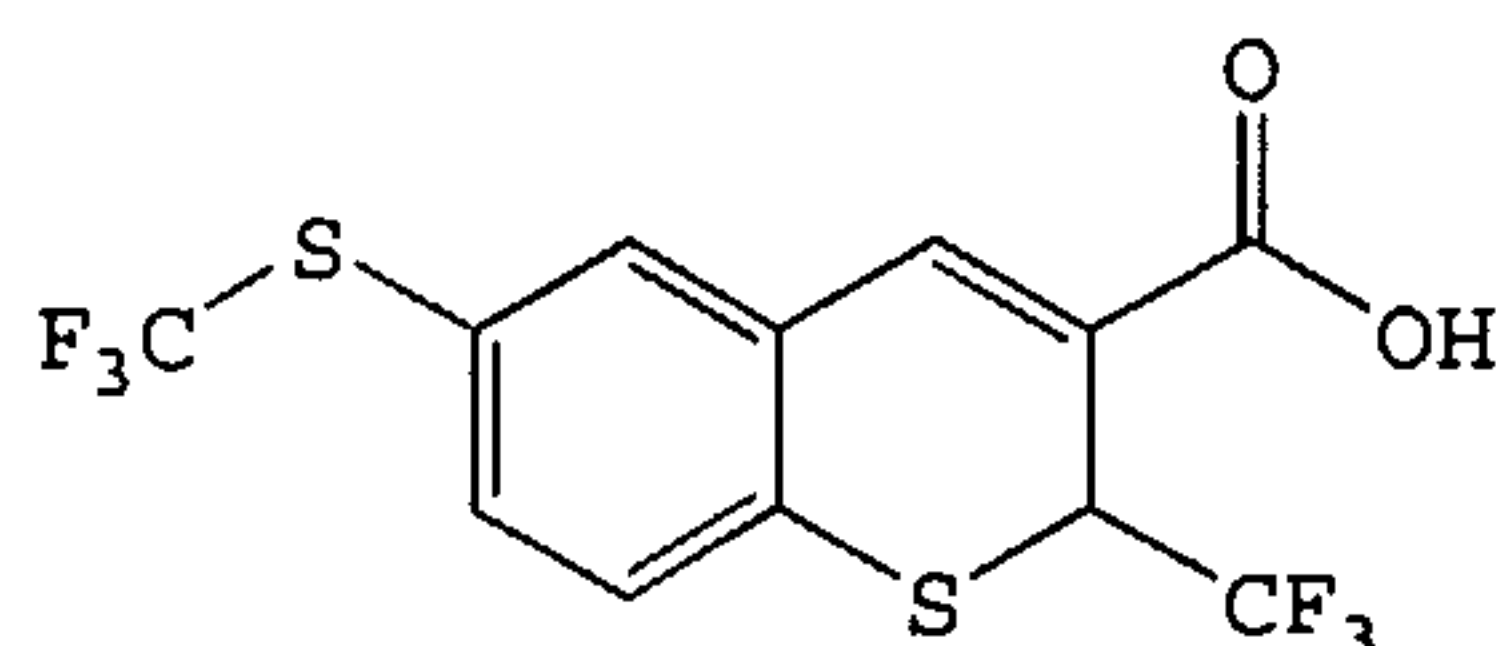
2-(Trifluoromethyl)-6-[(trifluoromethyl)thio]- 2H-1-benzothiopyran-3-carboxylic acid
