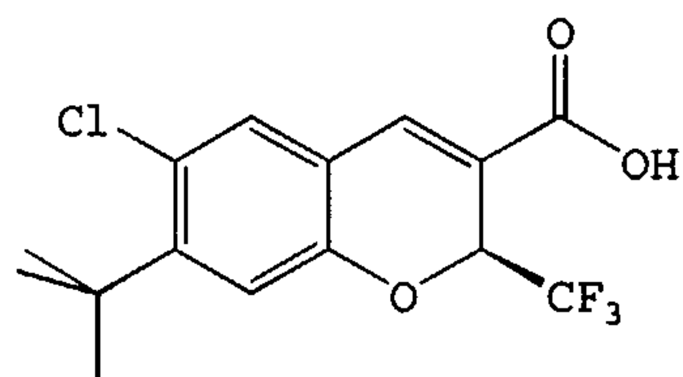
((S)-6-Chloro-7-(1,1-dimethylethyl)-2-(trifluoromethyl)-2H-1-benzopyran-3-carboxylic acid
