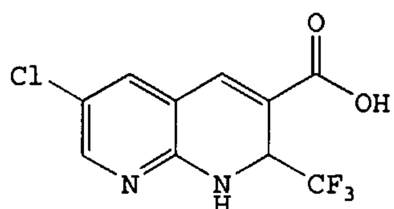
6-Chloro-2-(trifluoromethyl)-1,2-dihydro [1,8]naphthyridine-3-carboxylic acid
