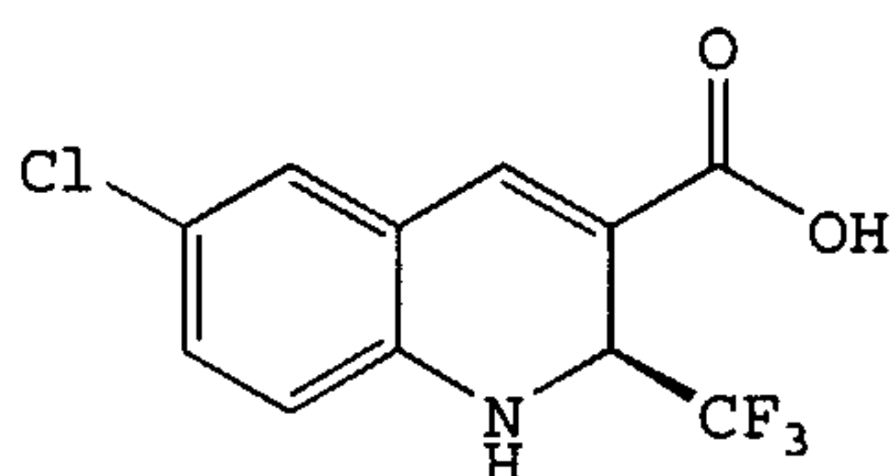
((S)-6-Chloro-1,2-dihydro-2-(trifluoro methyl)-3-quinolinecarboxylic acid
