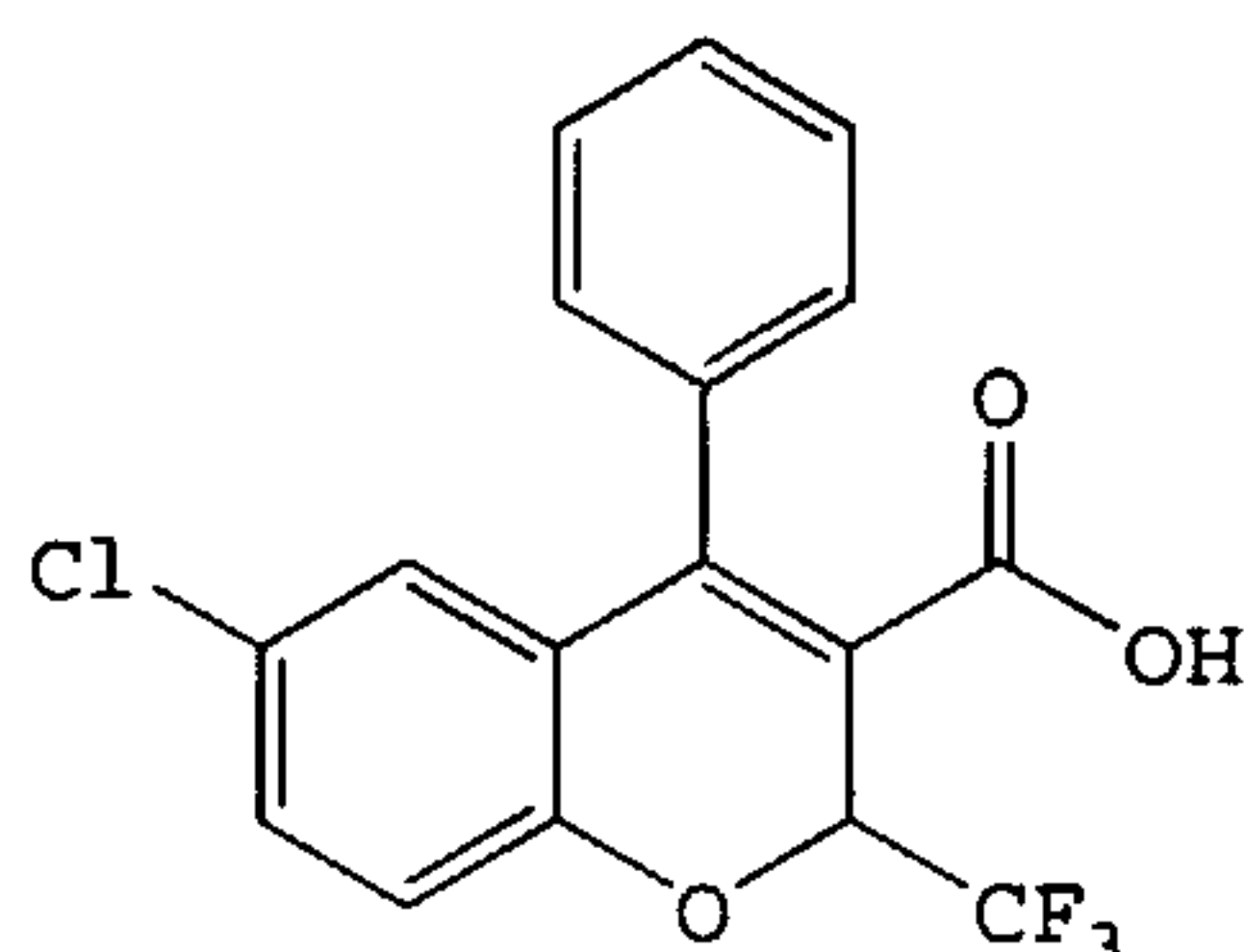
6-Chloro-2-(trifluoromethyl)-4-phenyl-2H- 1-benzopyran-3-carboxylic acid
