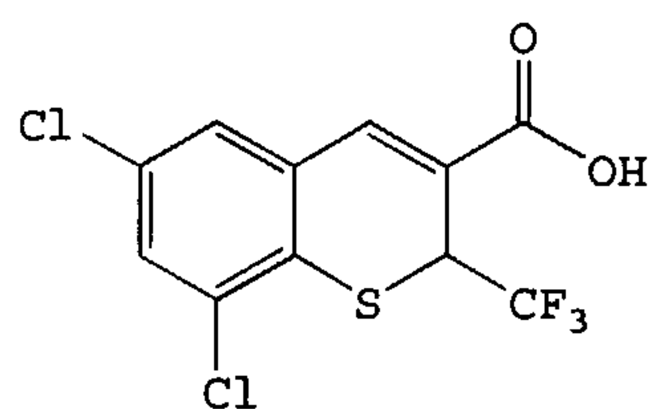
6,8-Dichloro-2-trifluoromethyl-2H-1- benzothiopyran-3-carboxylic acid
