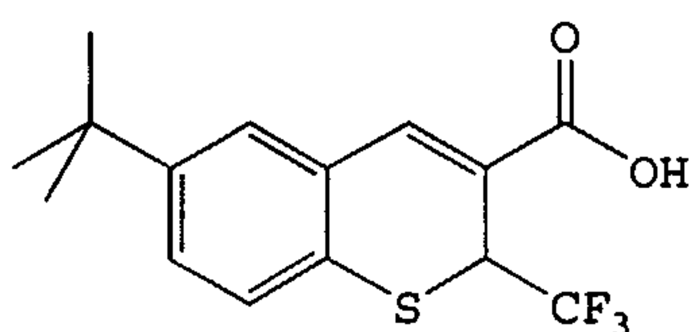
6-(1,1-Dimethylethyl)-2-(trifluoromethyl)-2H-1-benzothiopyran-3-carboxylic acid
