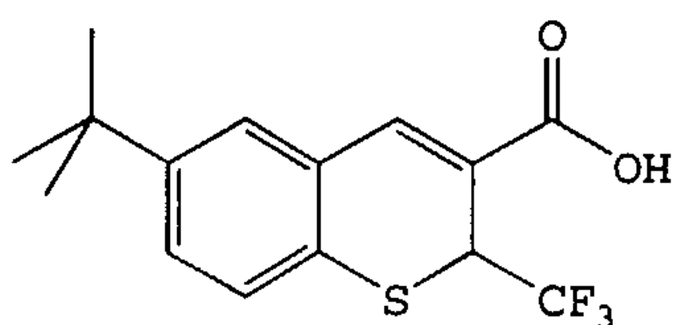
6-(1,1-Dimethylethyl)-2-(trifluoromethyl) -2H-1-benzothiopyran-3-carboxylic acid
