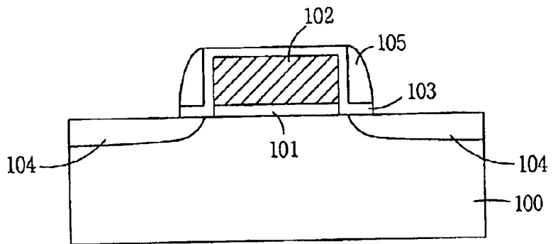
FIG. 1C BACKGROUND ART
