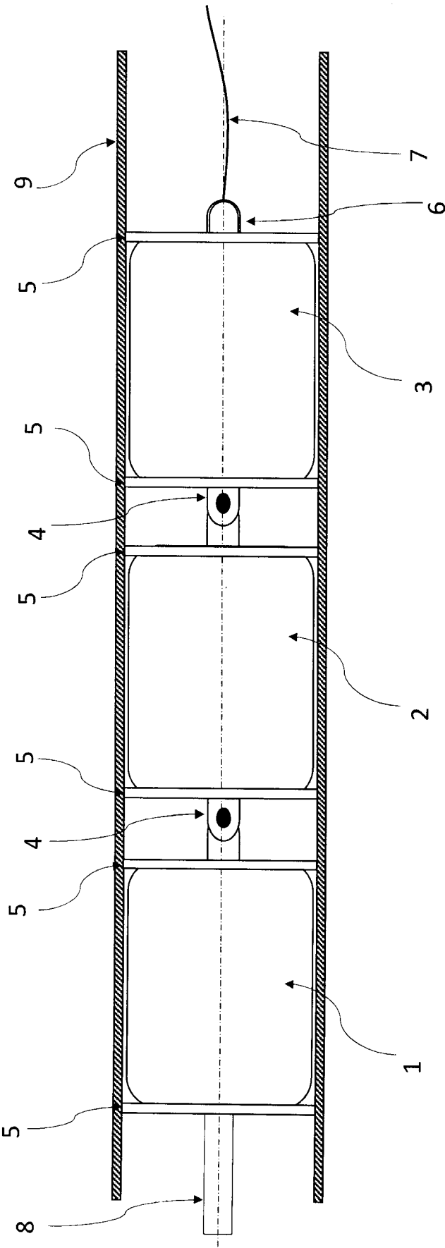
Exemplar of a Tool with Multiple Modules within a Tubular with Push and/or Pull Propulsion Capabilities
