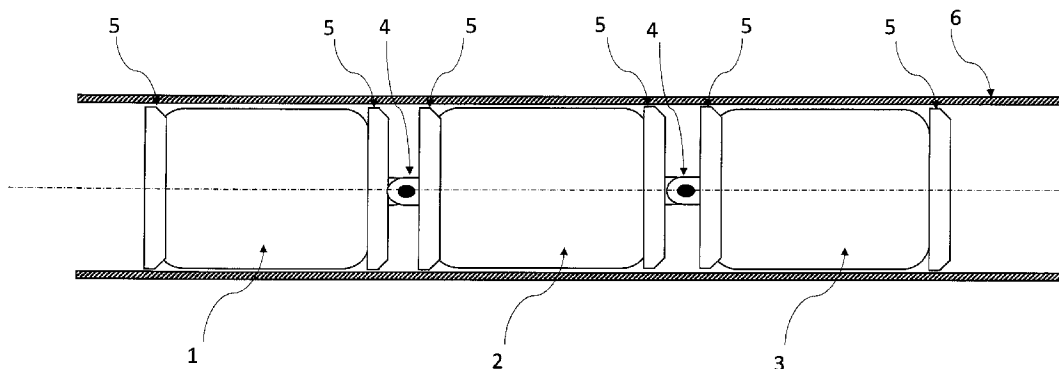
Exemplar of a Tool with Multiple Modules within a Tubular
