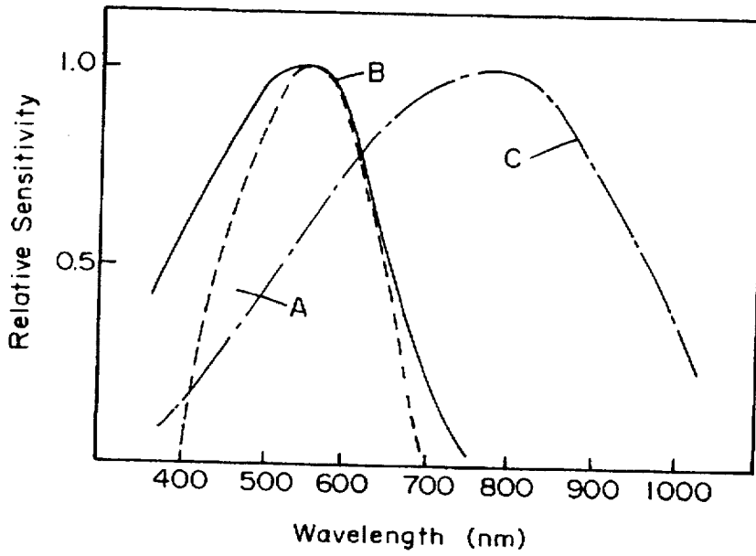
FIG. 7 PRIOR ART
