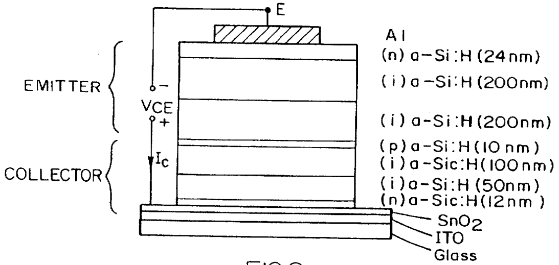
FIG. 9 PRIOR ART
