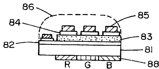
FIG. 8(c) PRIOR ART
