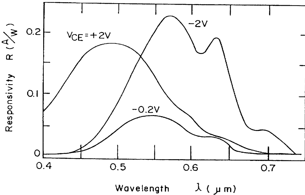
FIG. 10 PRIOR ART
