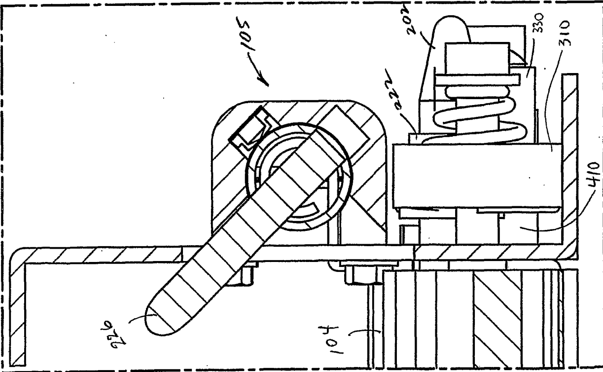
DETAIL B FIG. 5C
