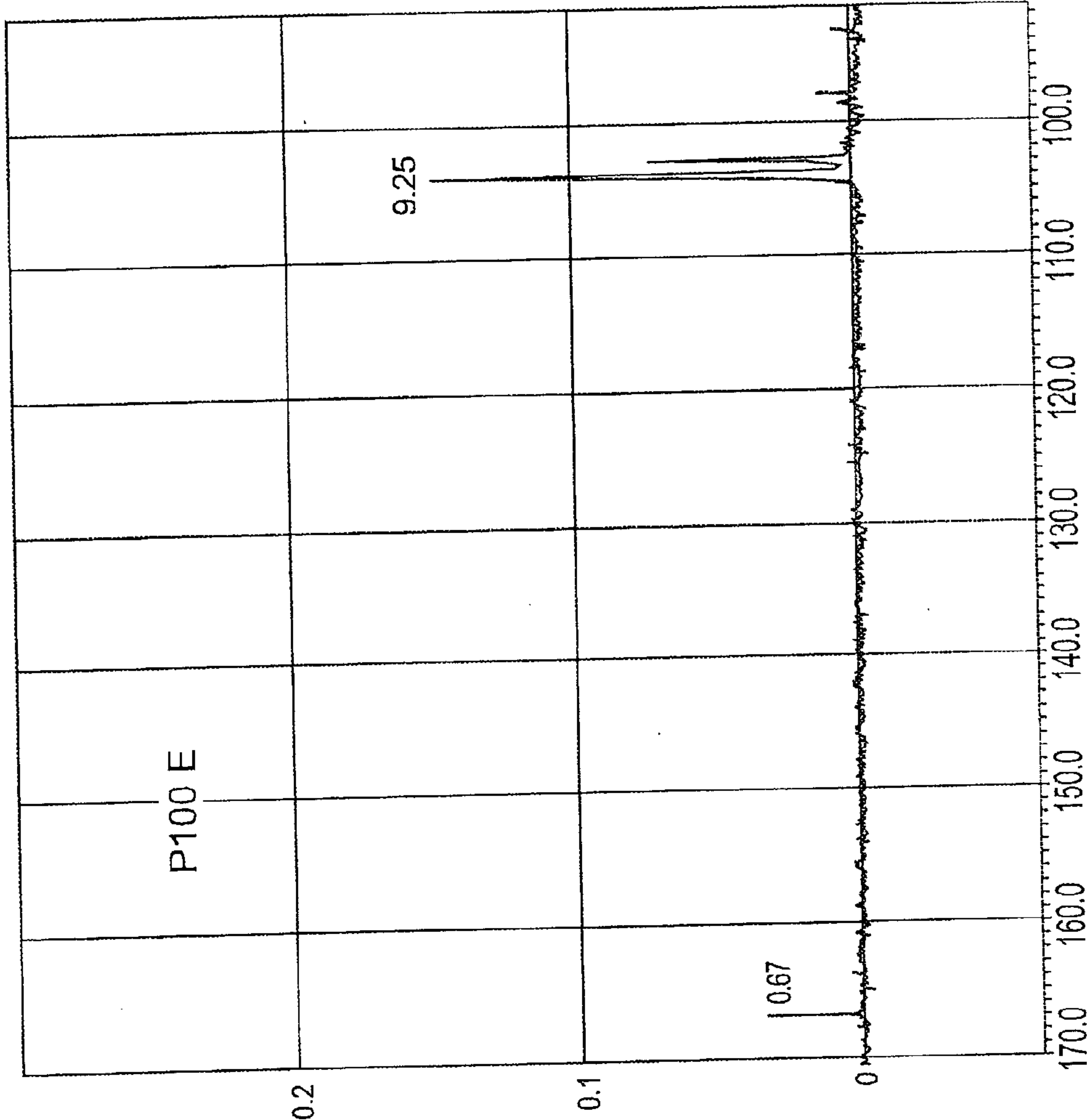
FIG. 40M X : parts Per Million : 13C
