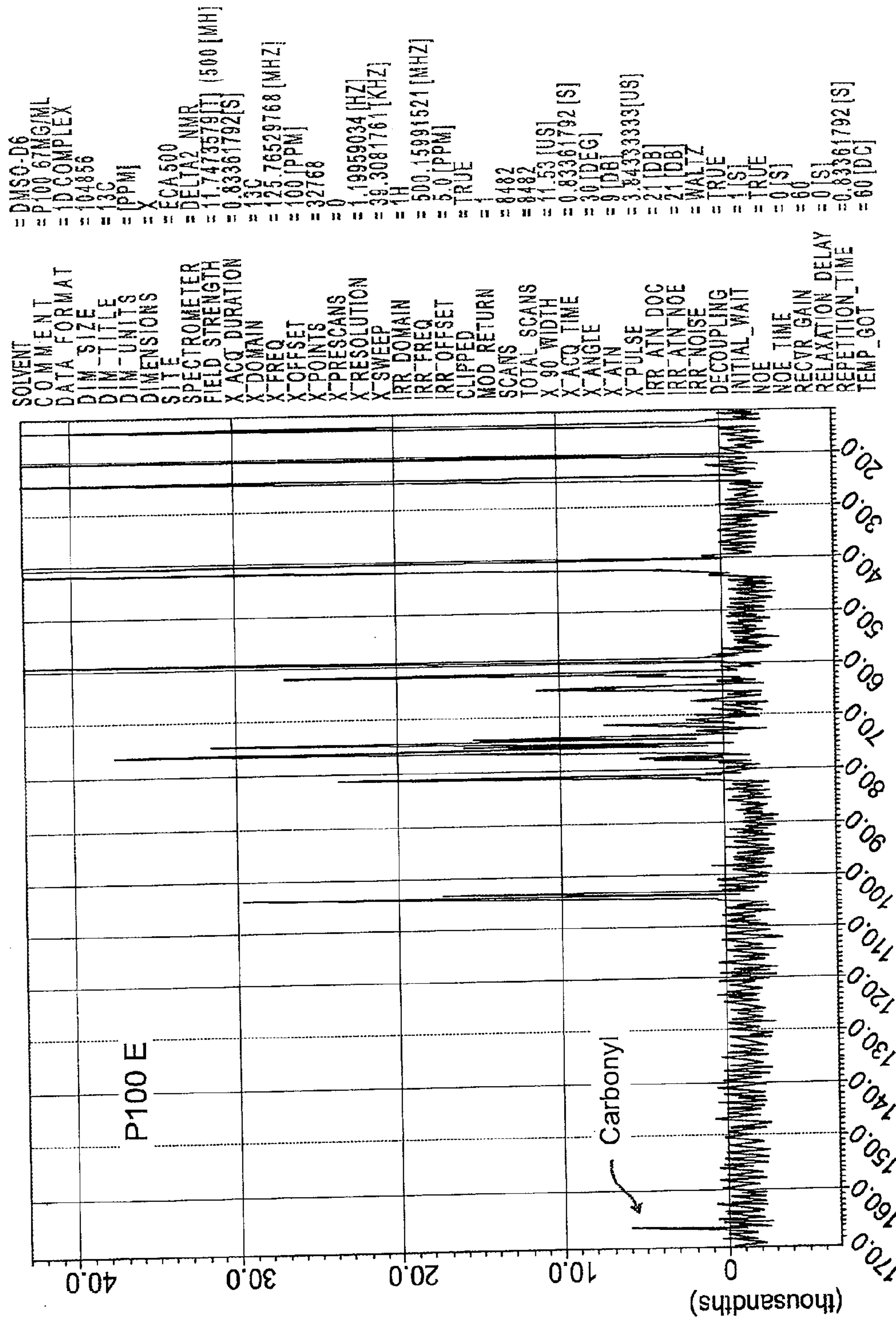
FIG. 40 K X : parts per Million : 13C
