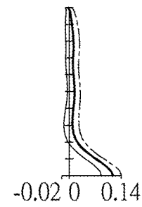
Sagittal field curvature
