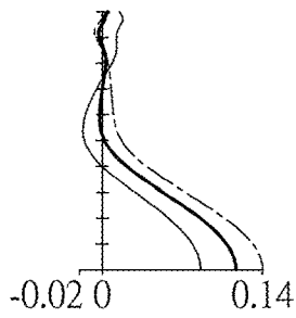
Longitudinal spherical aberration
