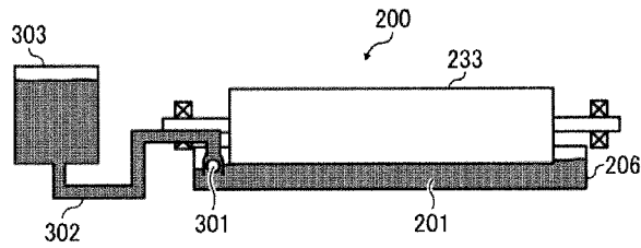
FIG. 11 RELATED ART
