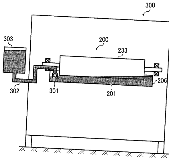
FIG. 12 RELATED ART
