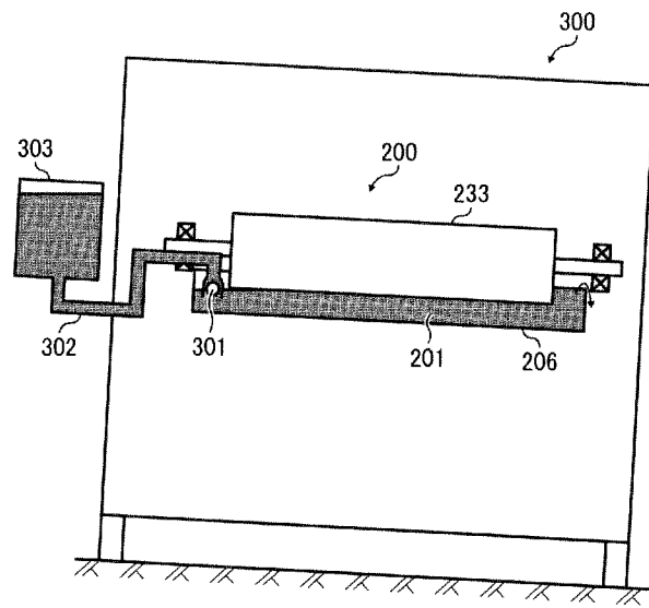
FIG. 13 RELATED ART
