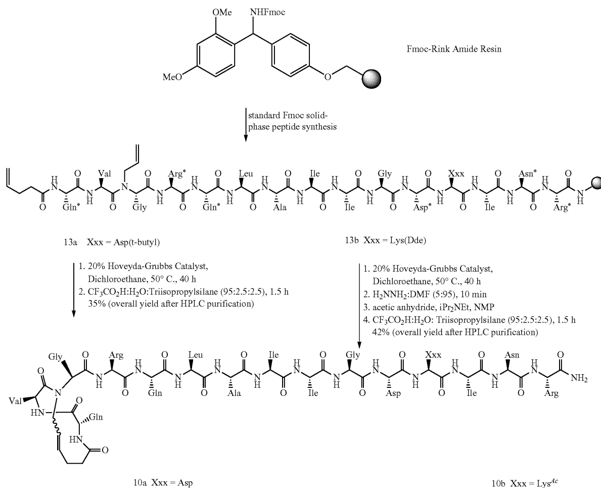
Scheme 12
