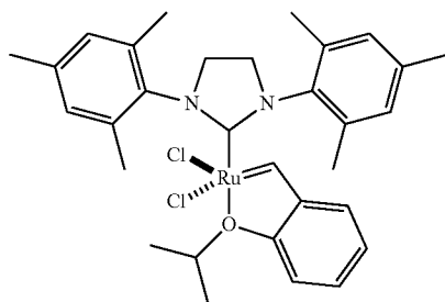
Hoveyda-Grubbs Catalyst
