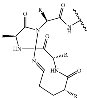
hydrazone approach
