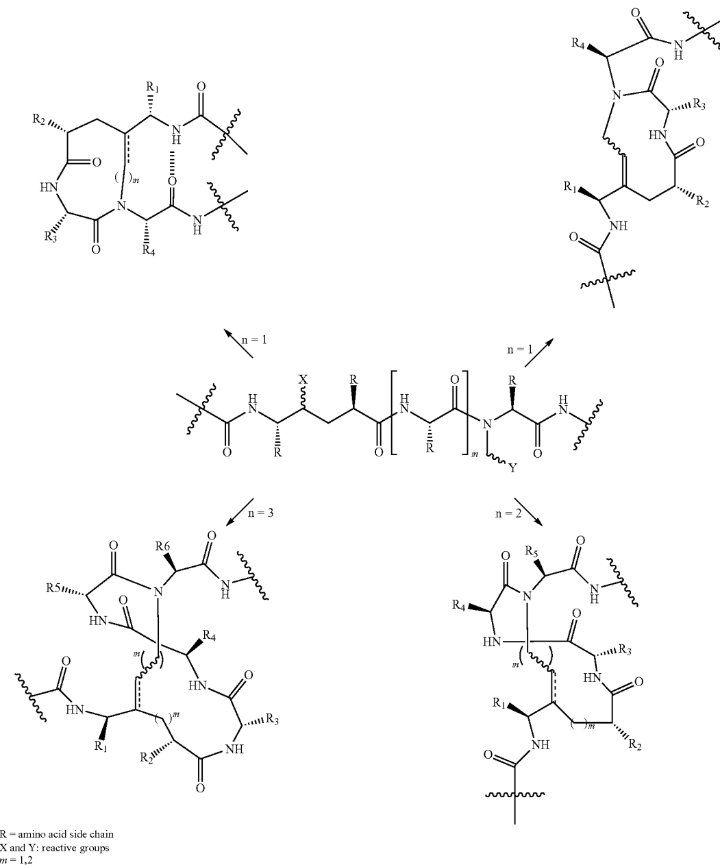
Scheme 8
