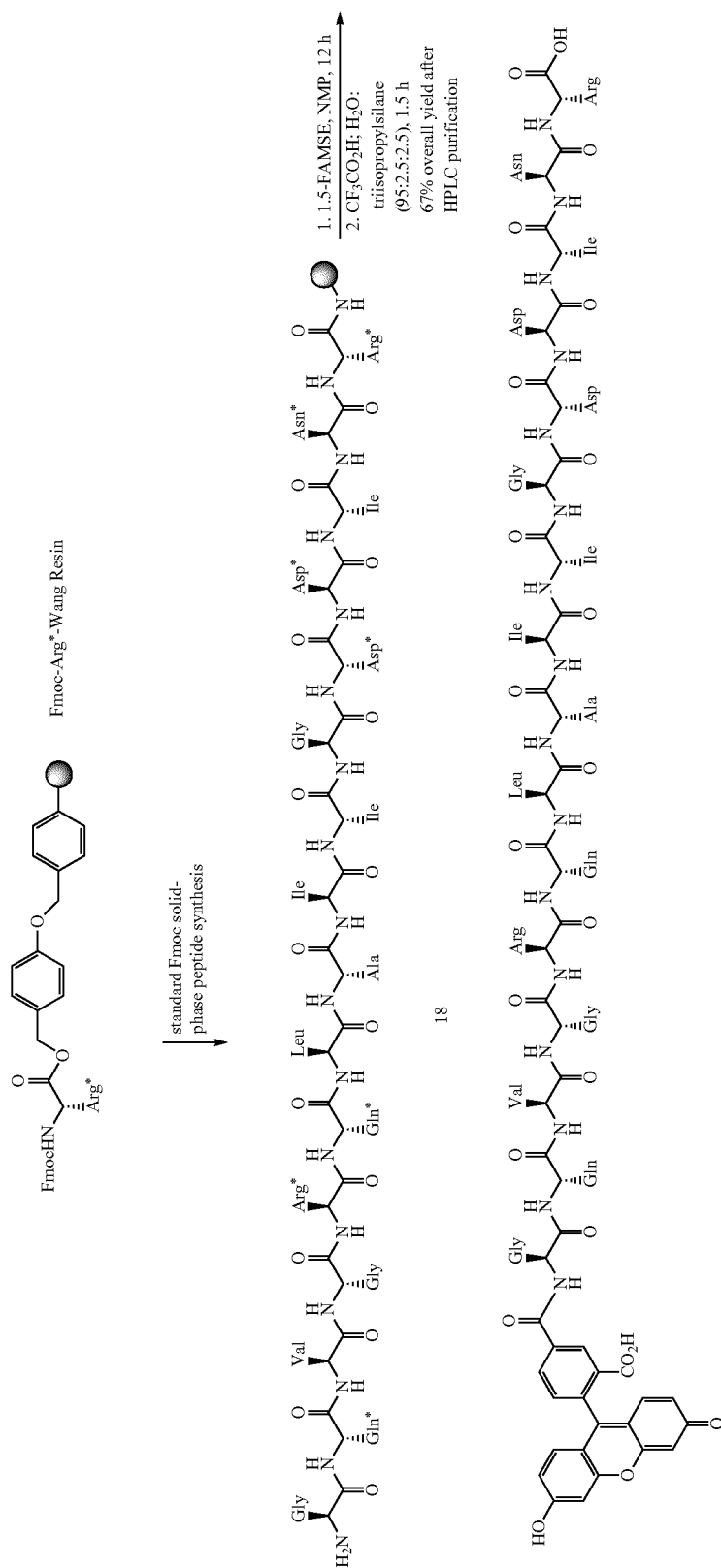
Scheme 13
