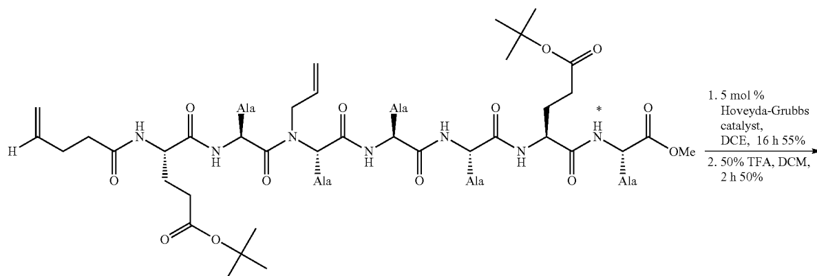
Scheme 7
