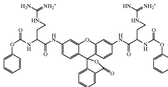
(CBZ-arginine) 2 rhodamine 110
