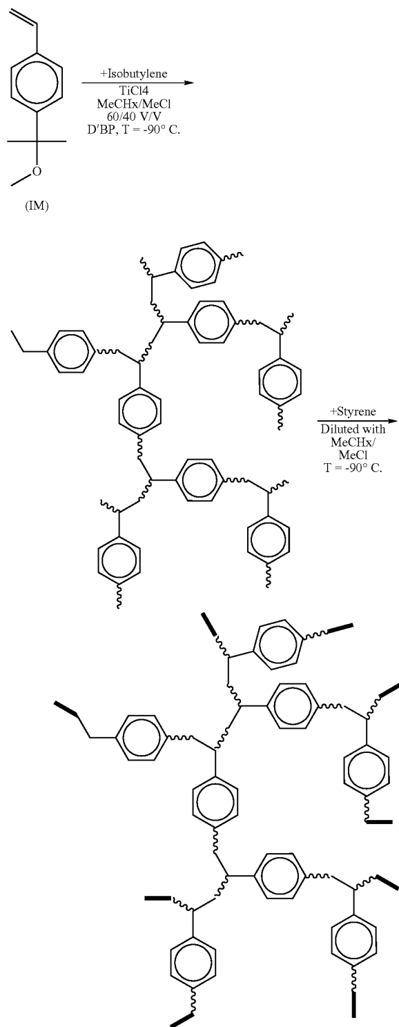
Scheme 1
