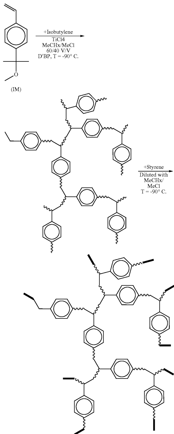
Scheme 1
